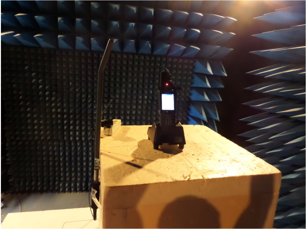
Anechoic chamber
