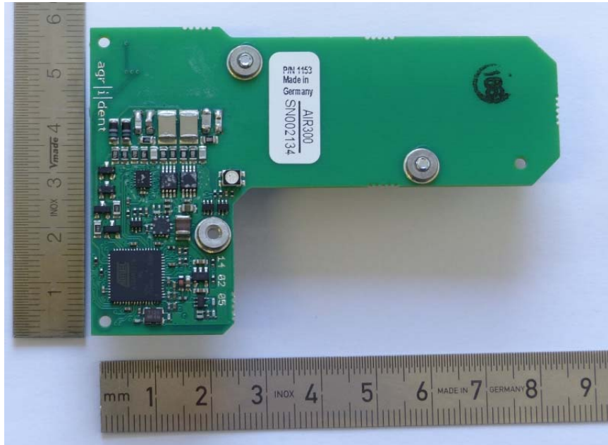
AIR300 PCB Top Side:
