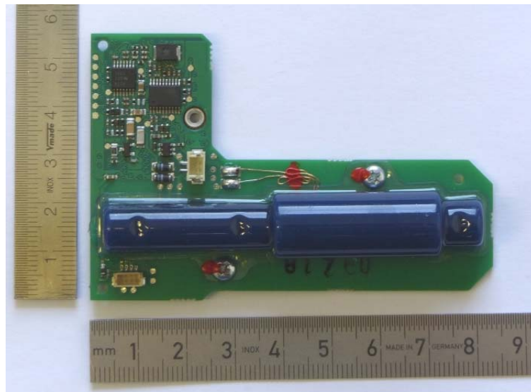
AIR300 PCB Bottom Side:
