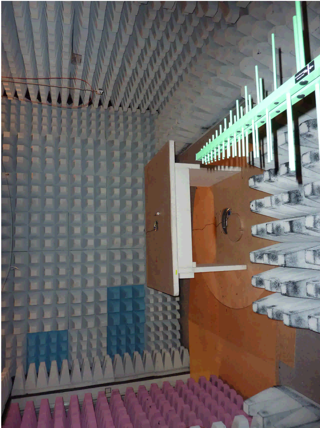
100853_30.jpg ABR105, test set-up fully anechoic chamber
