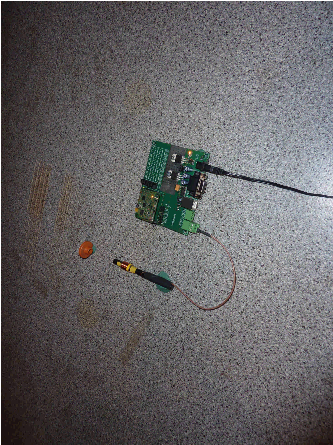
100853_38.jpg ABR105, test set-up fully anechoic chamber
