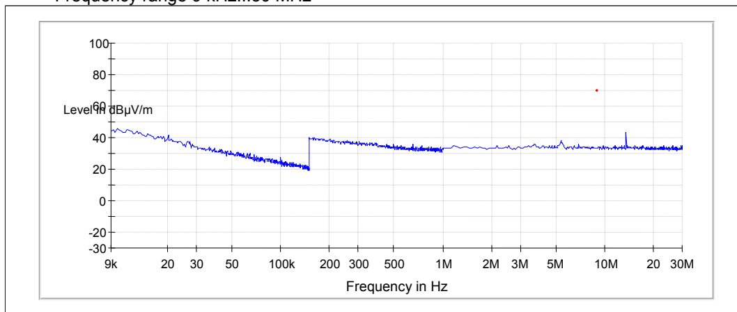
Frequency range 9 kHz...30 MHz
