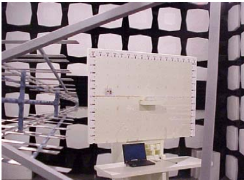
Picture 3. FCC Part 15B Radiated emissions
