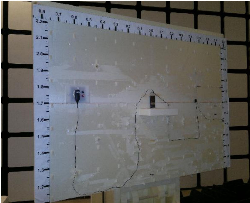
Picture 1. FCC Part 15C Radiated emissions
