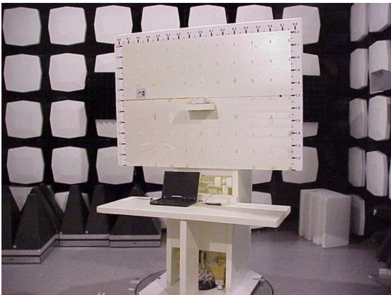
Picture 2. FCC Part 15B Radiated emissions
