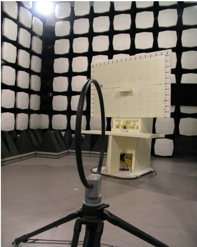
Picture 2. FCC Part 15C Radiated emissions
