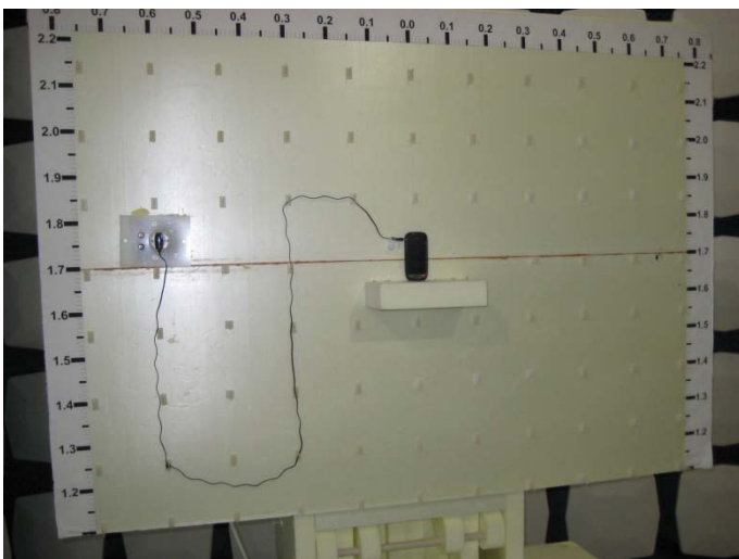
Picture 2. FCC Part 15C Radiated emissions, FM TX
