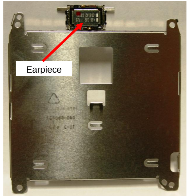
Display Chassis Rear
