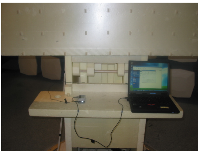
Picture 2 Radiated emission measurement GSM RX / Bluetooth TX + Computer peripherals
