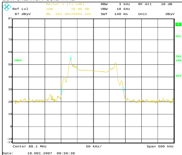
Low channel / 88.1 MHz
