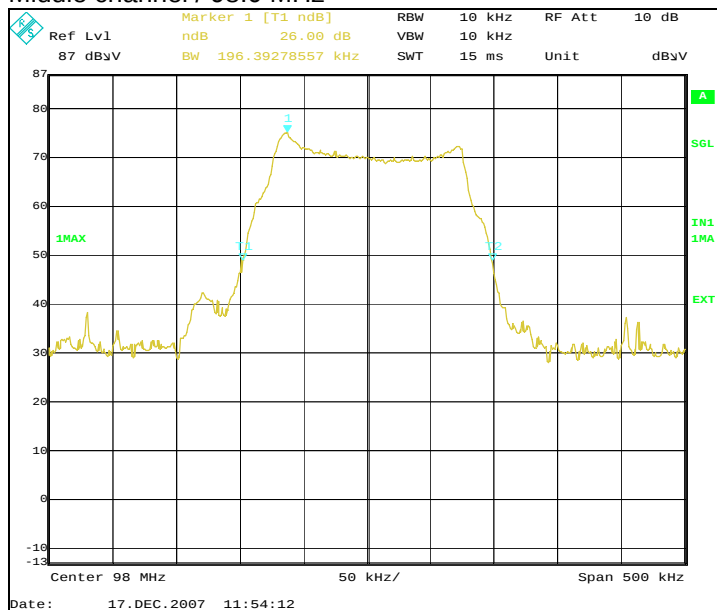
Middle channel / 98.0 MHz
