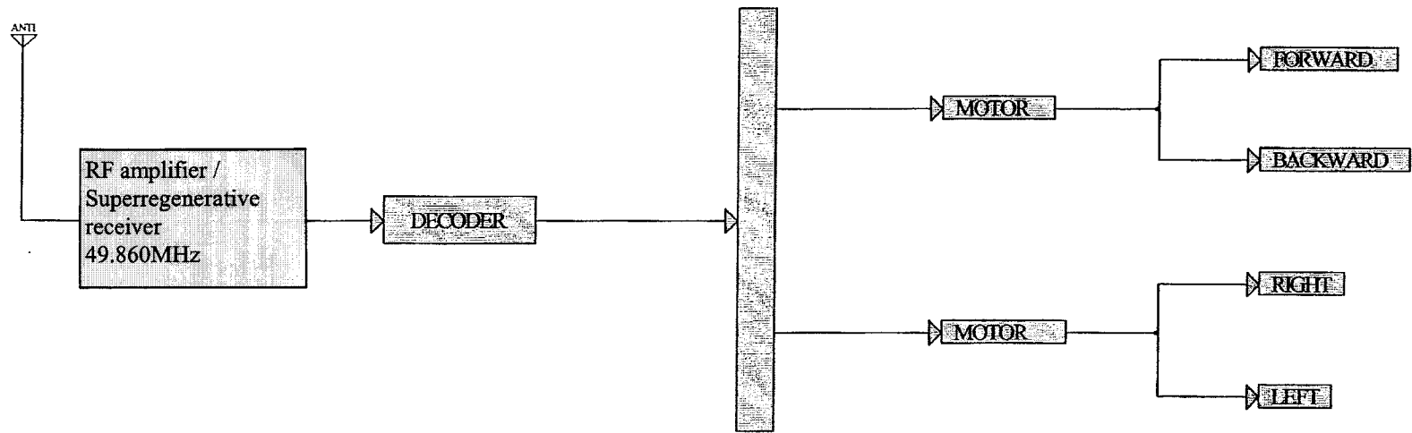
RX-49.860MHZ FUNCTION BLOCK DIAGRAM
