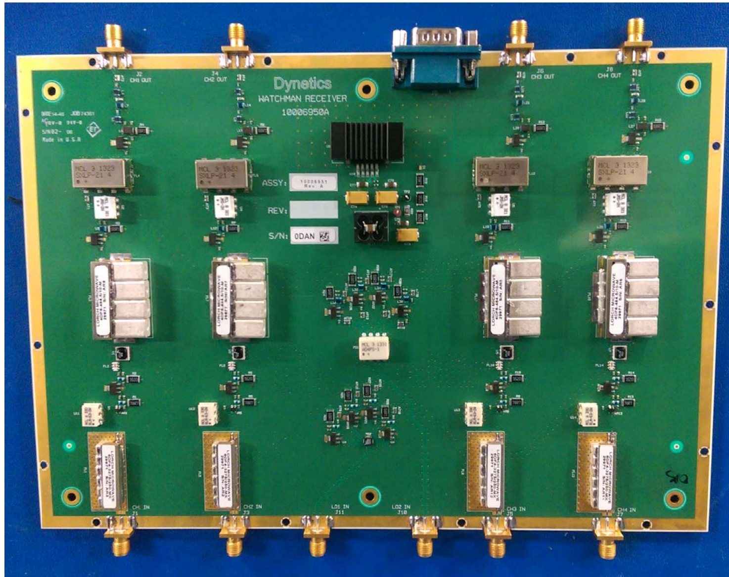
RF Receiver Board (2 Per Unit) Top View
