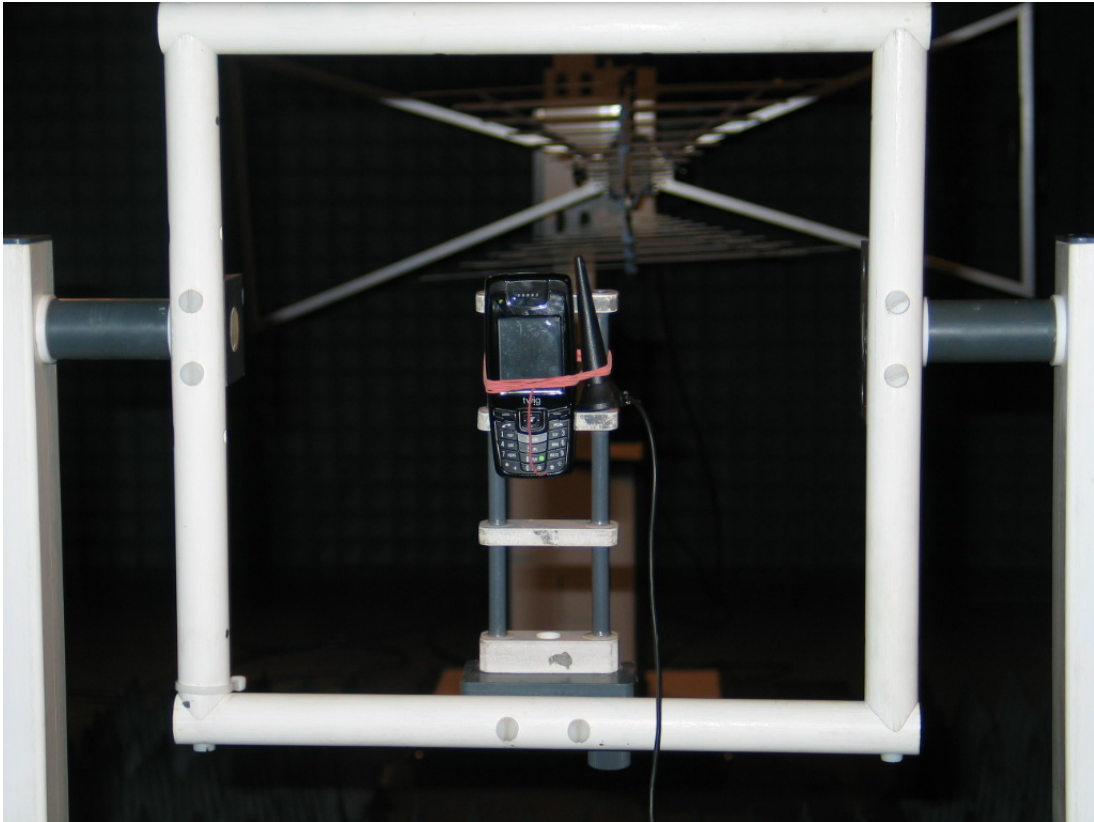
PHOTO No. 3: Setup used for radiated measurements
