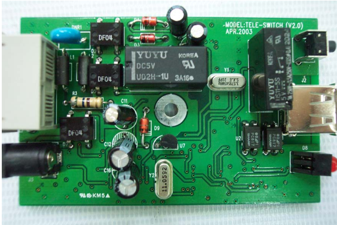
Main board
