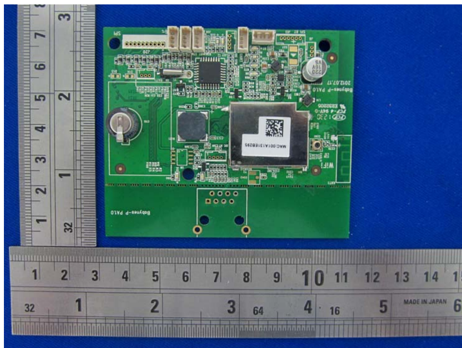
EUT Top View without Shielding
