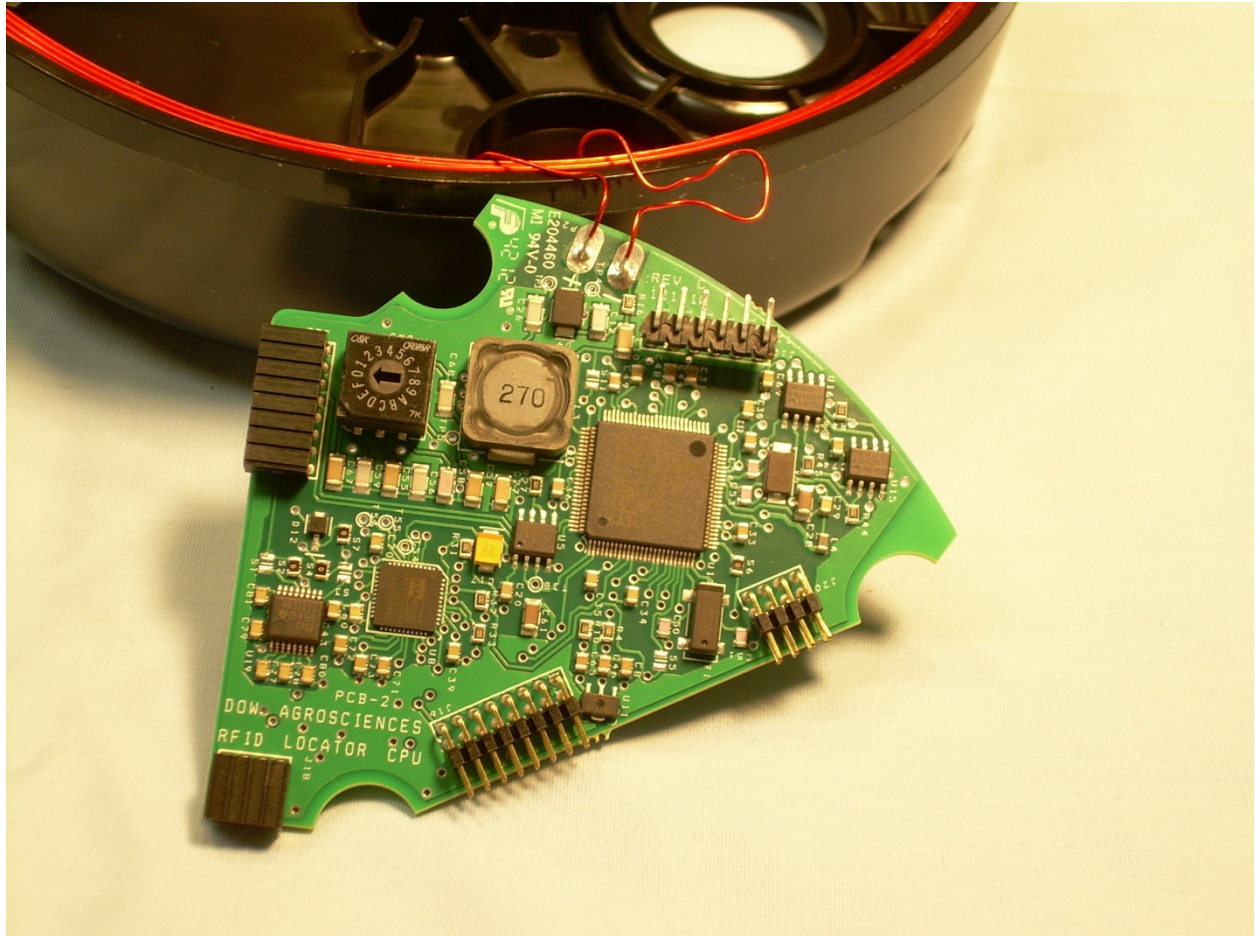
Top View of PCB #2
