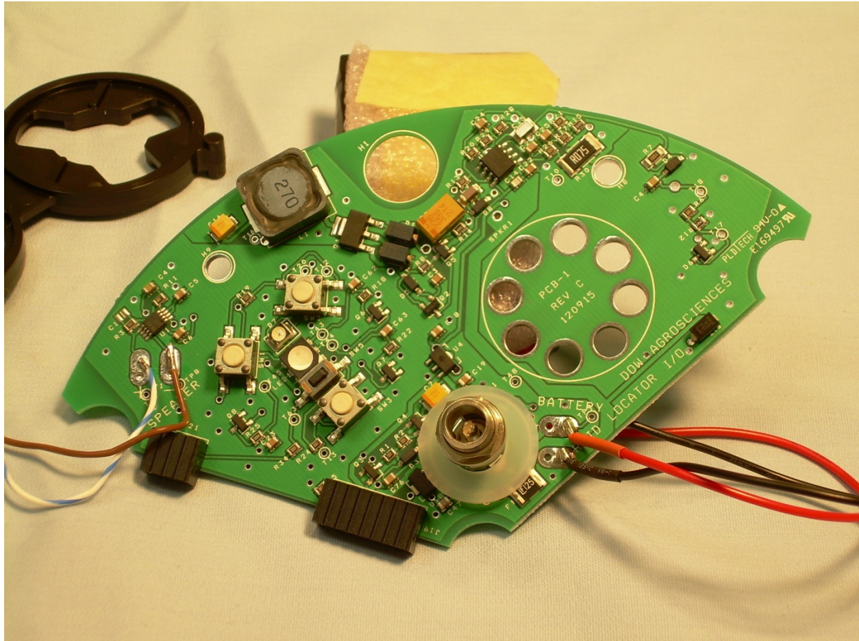
Top View of PCB #1
