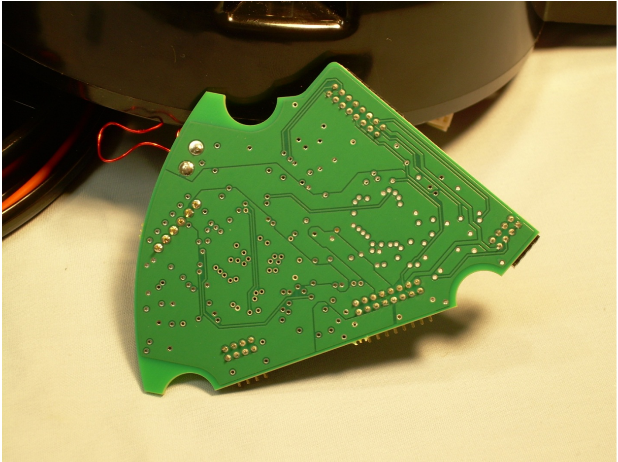
Bottom View of PCB #2
