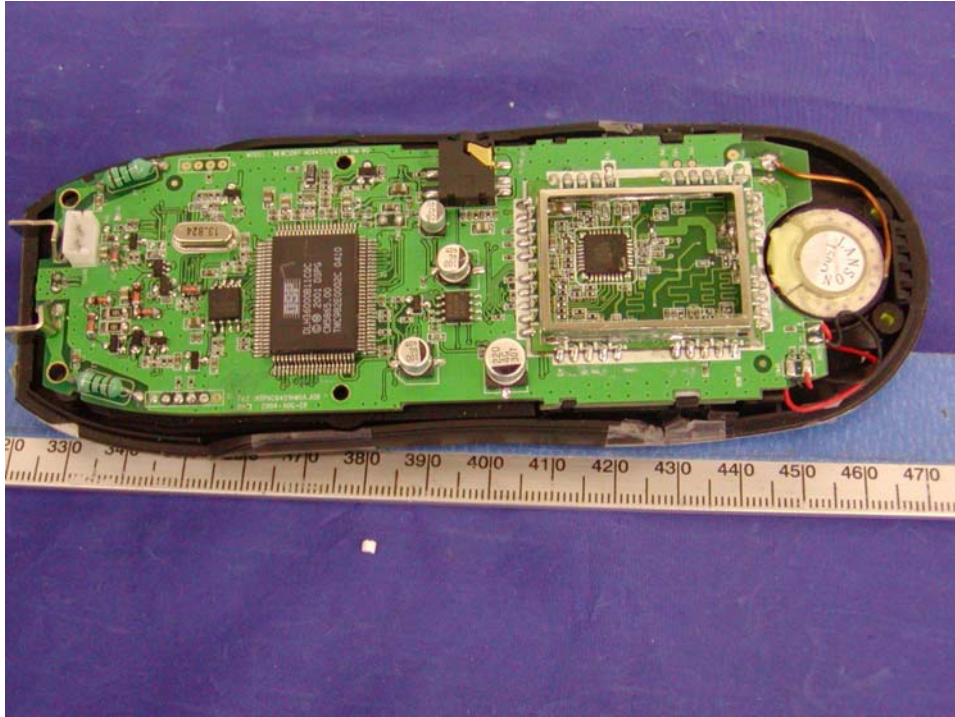
Handset – Chassis Cover off View
