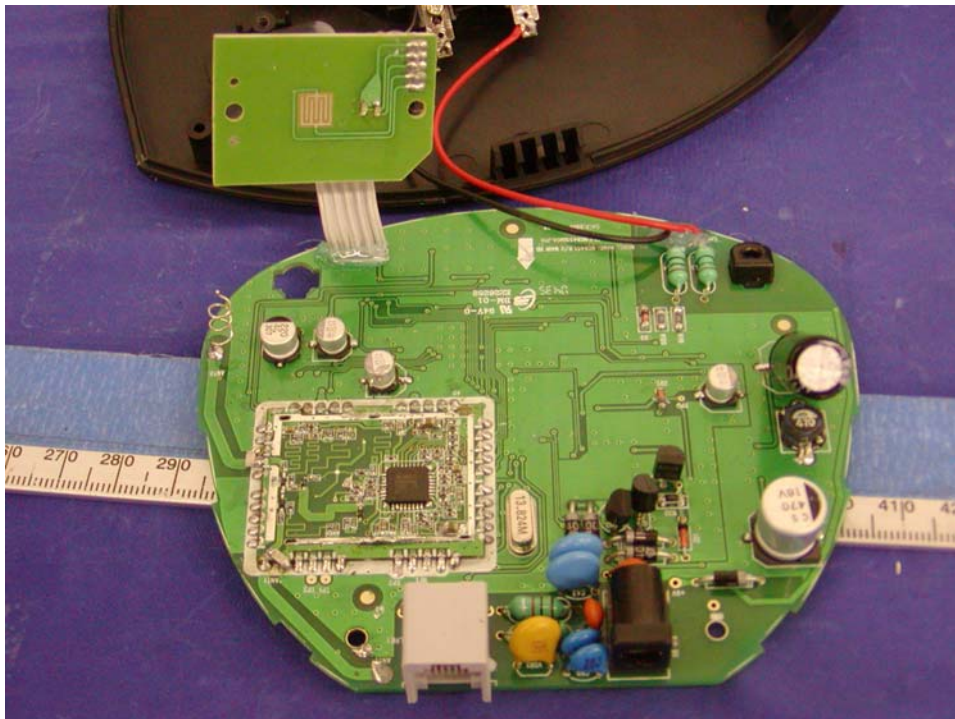
Base – Component View
