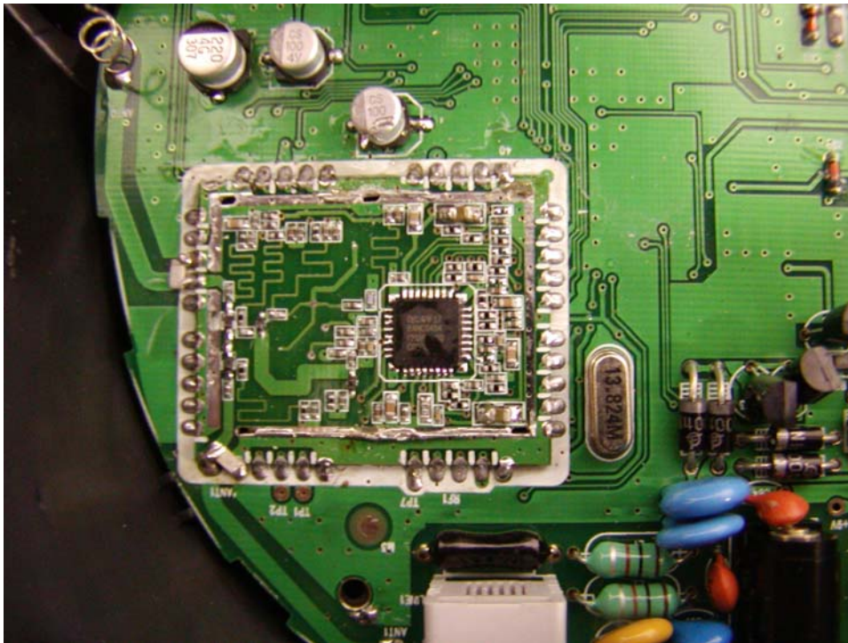
Base – Transceiver View
