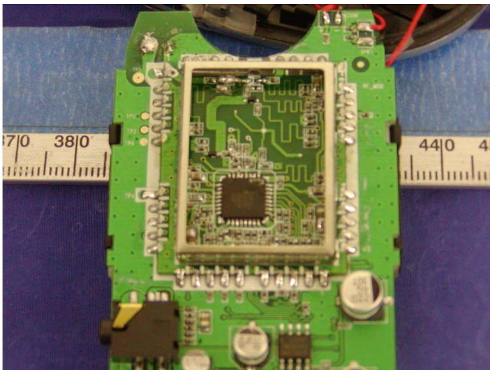
Handset - Transceiver View
