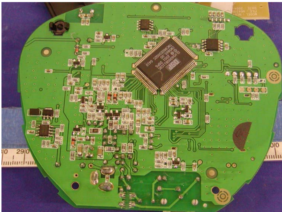
Base – Solder View
