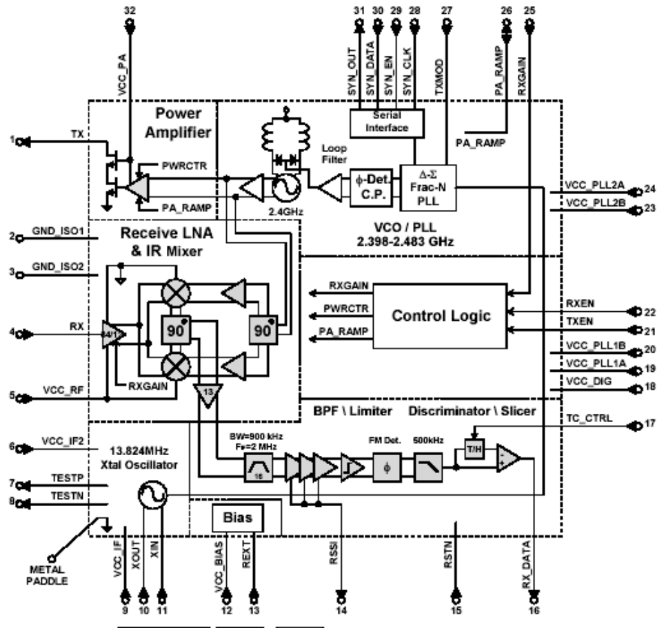
RFIC BLOCK DIAGRAM
