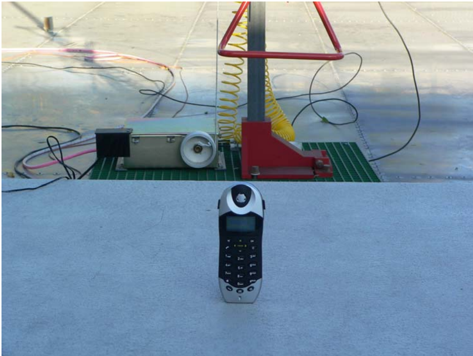
Radiated Emission - Front View for Handset
