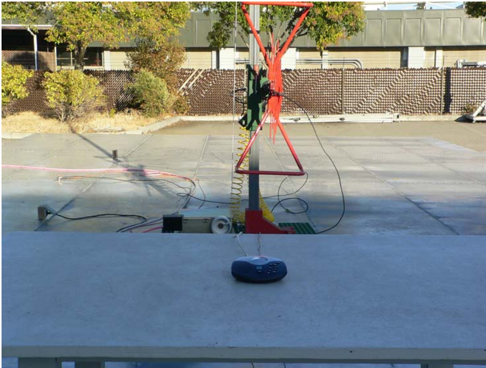
Radiated Emission - Front View for Base
