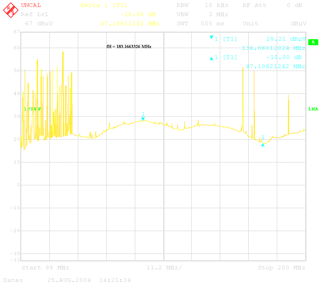
FIGURE 3.2-1A 5104 10dB BANDWIDTH
