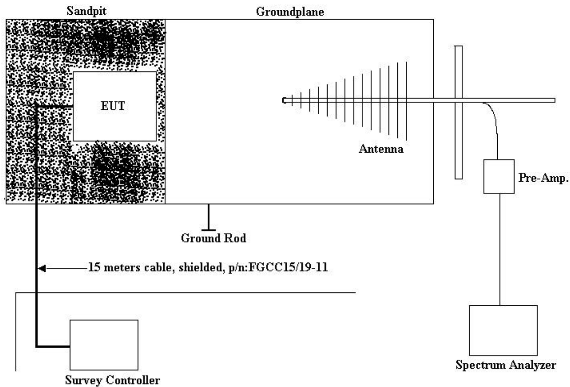
FIGURE 1.3-1 TEST SETUP BLOCK DIAGRAM (M/N 5104)
