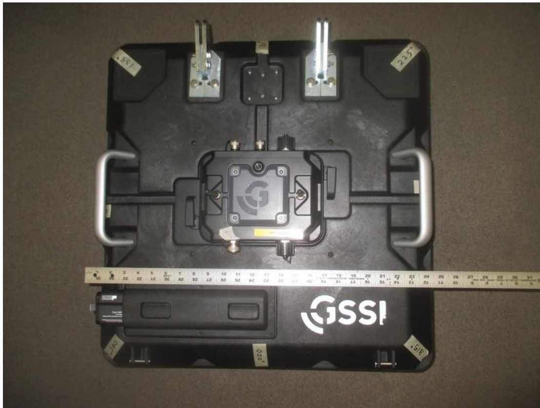
EUT_ Top View & Dimension (1)
