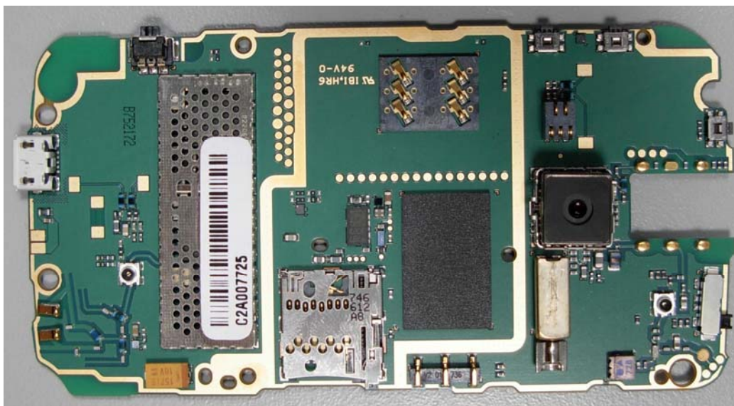
Fig 1 – PWB Back View: Shield in place
