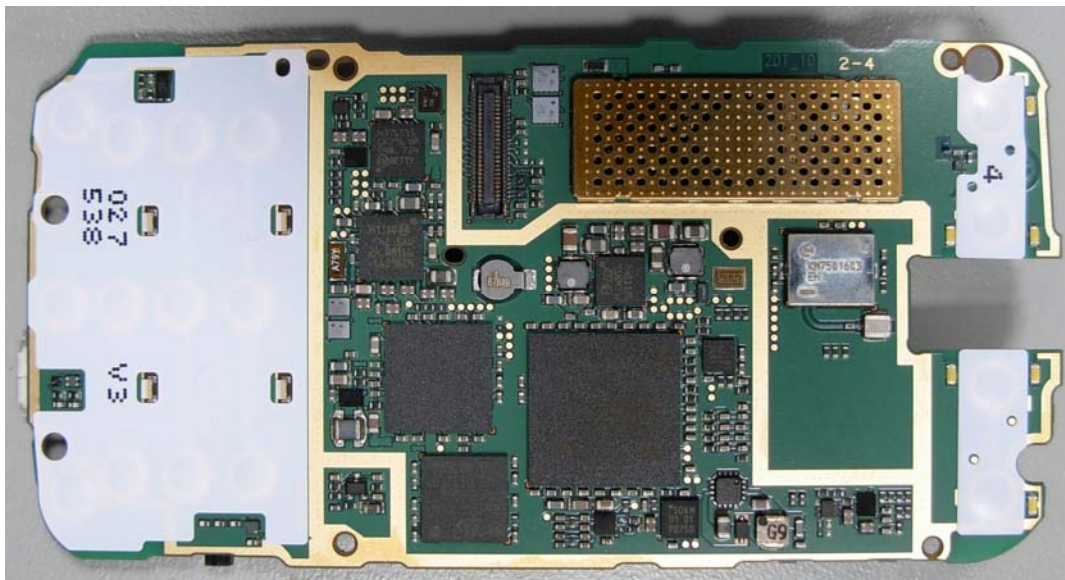
Fig 3 – PWB Front View: Shield in place
