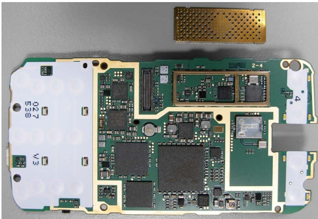
Fig 4 – PWB Front View: Shield removed
