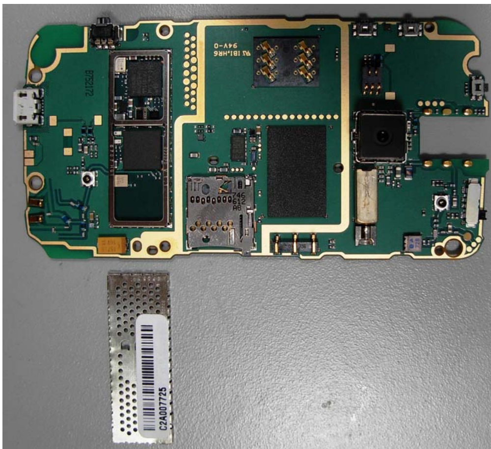
Fig 2 – PWB Back View: Shield removed
