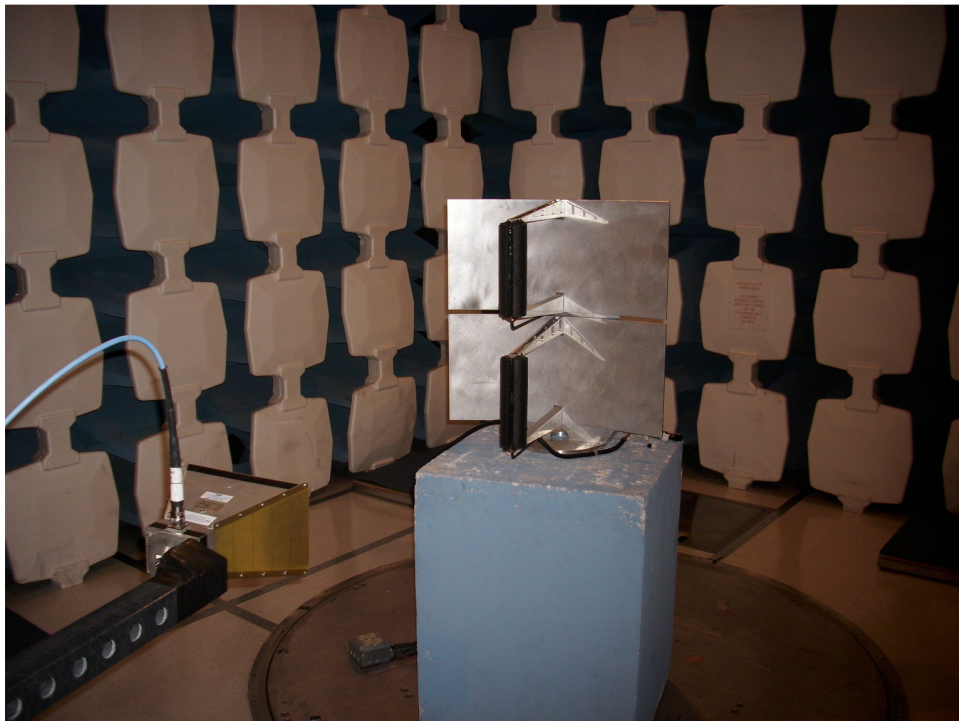
Radiated Measurements – 1 to 18GHz – Anechoic Chamber - Front
