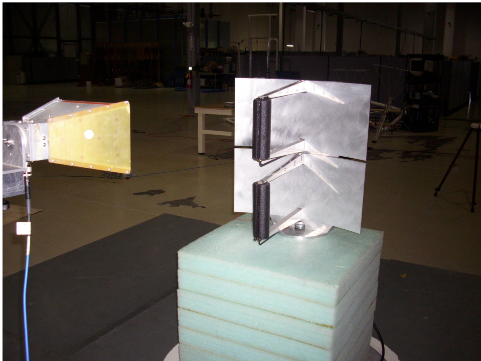
Radiated Measurements – 1 to 18GHz – OATS - Front
