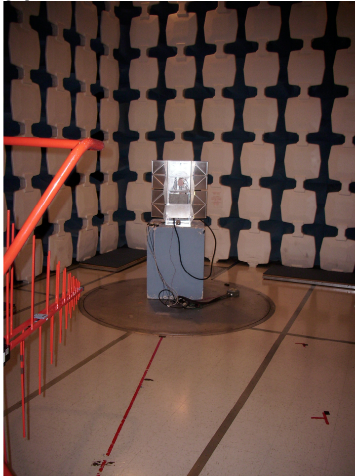
Radiated Measurements below 1GHz – Anechoic Chamber - Rear
