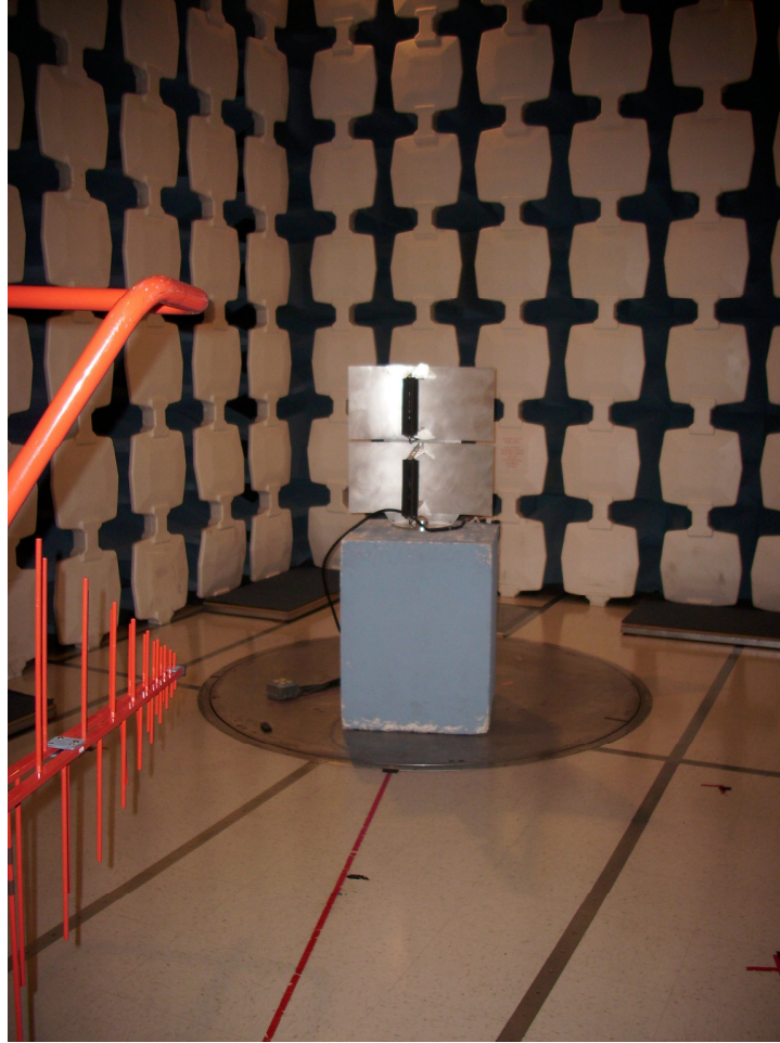
Radiated Measurements below 1GHz – Anechoic Chamber - Front
