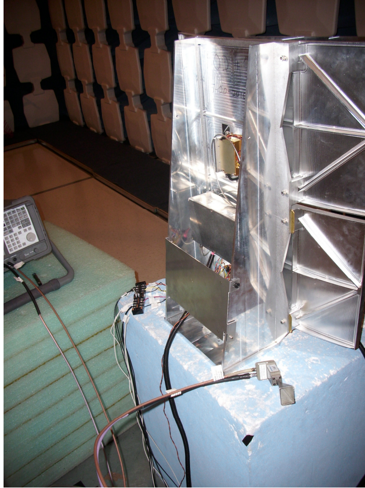
Radiated Measurements – Above 26.5GHz – Anechoic Chamber
