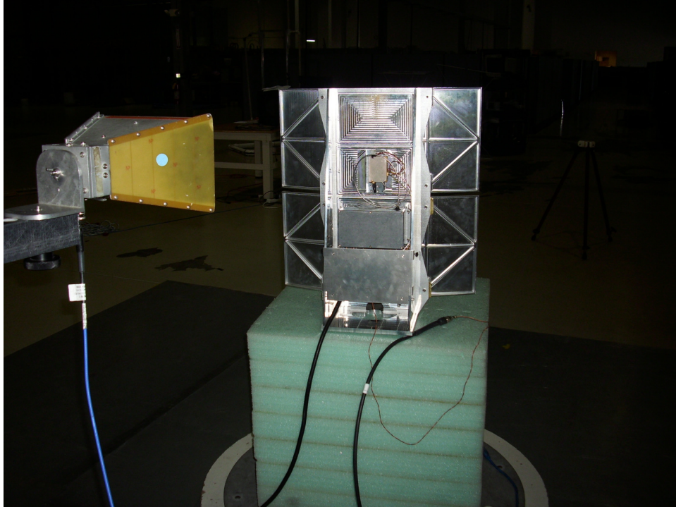
Radiated Measurements – 1 to 18GHz – OATS - Rear
