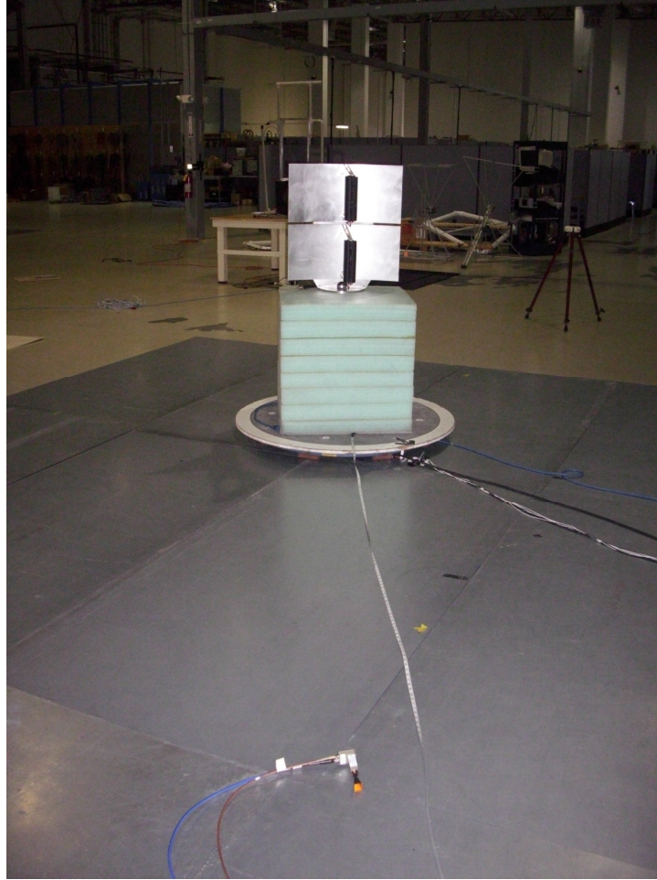
Radiated Measurements – Above 26.5GHz – OATS
