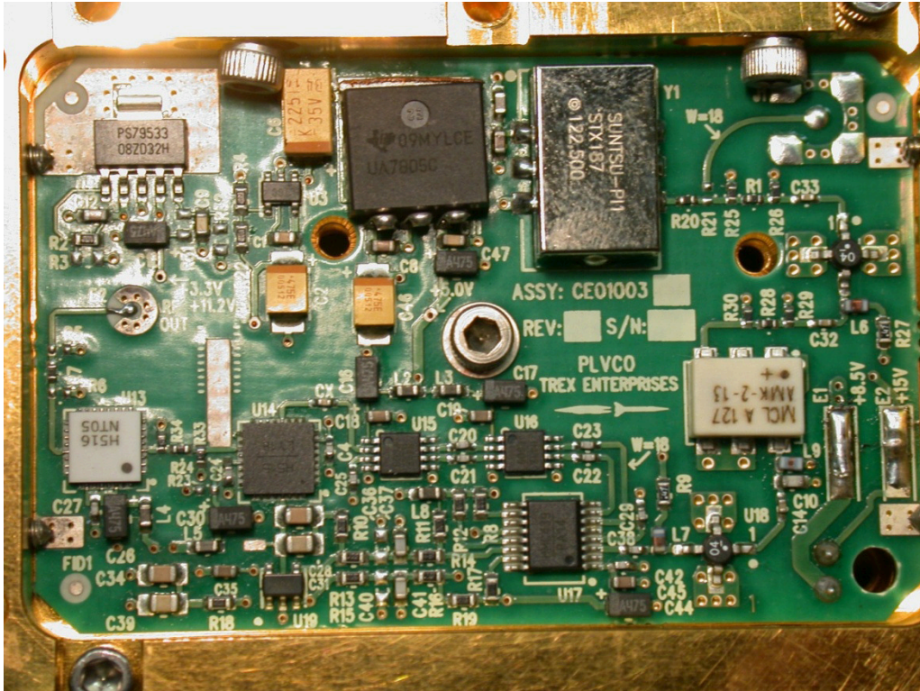
Tx Module with cover removed from back side Showing PLO circuit board
