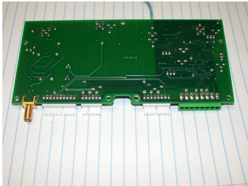
LSM board Rear side
