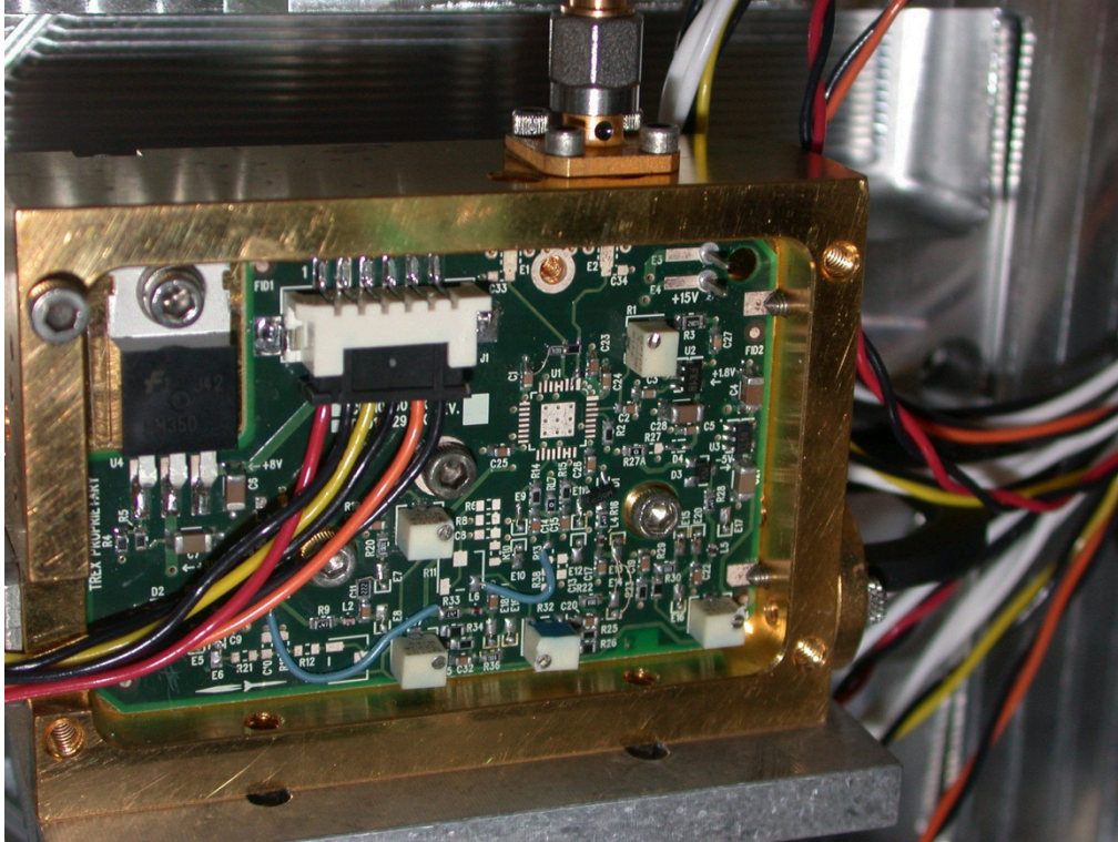
Tx Module Bias Board Front Side
