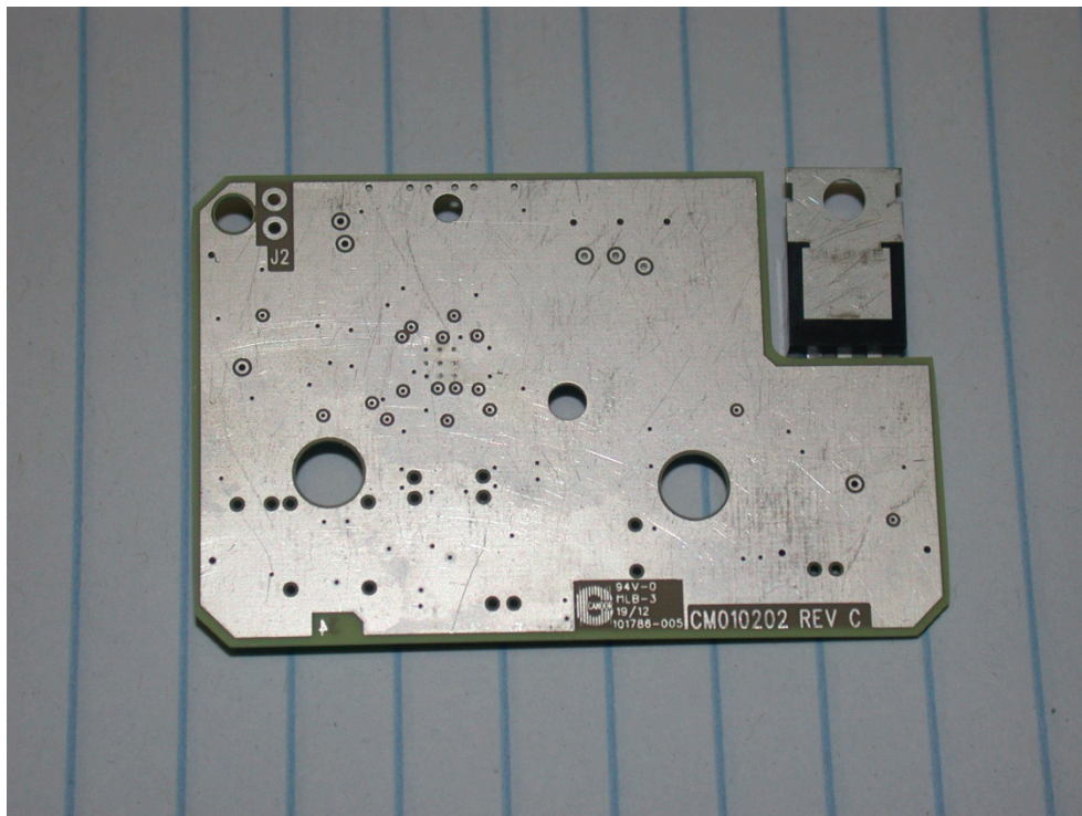
Tx Module Bias Board Rear Side
