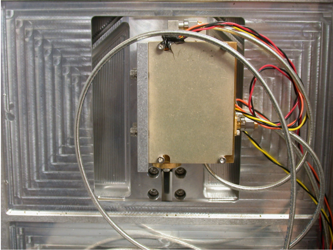
Receive Module with cover
