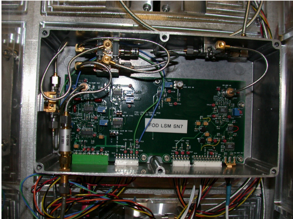
LSM module with cover removed no absorber
