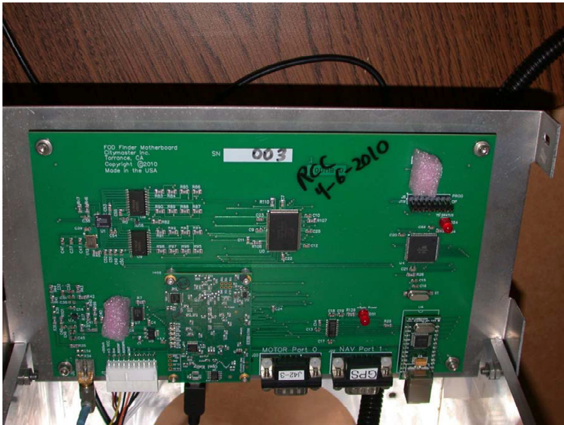
Control board Top Side
