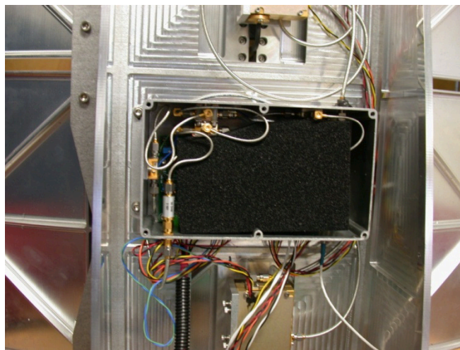
LSM with absorber LS-18-1/2
