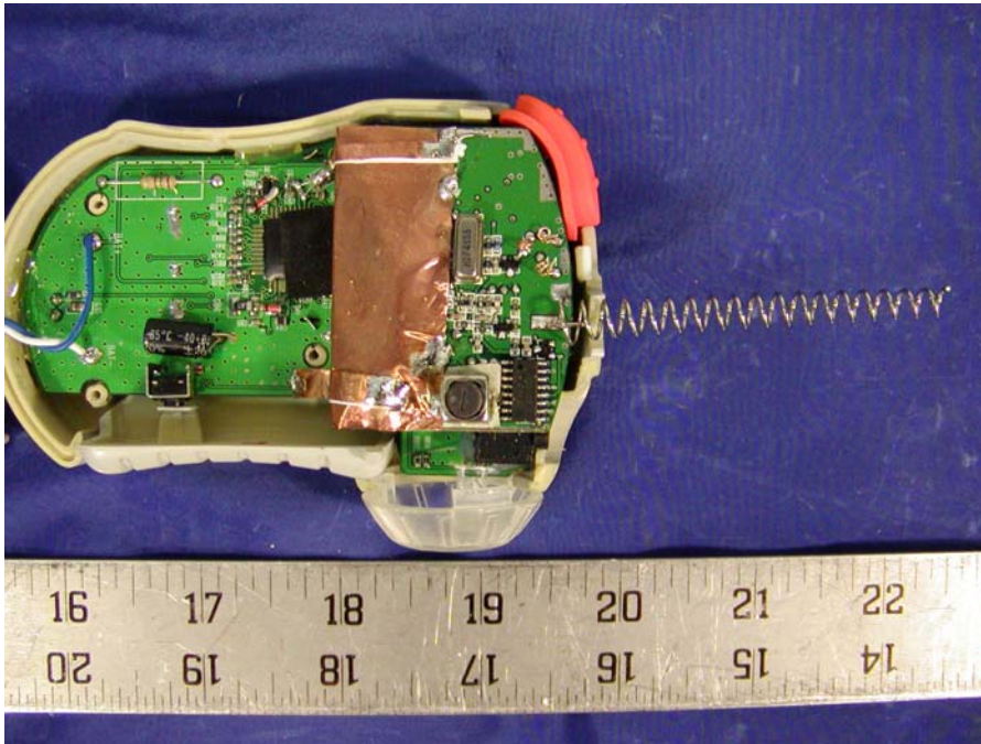
Antenna with its attachment on the PCB
