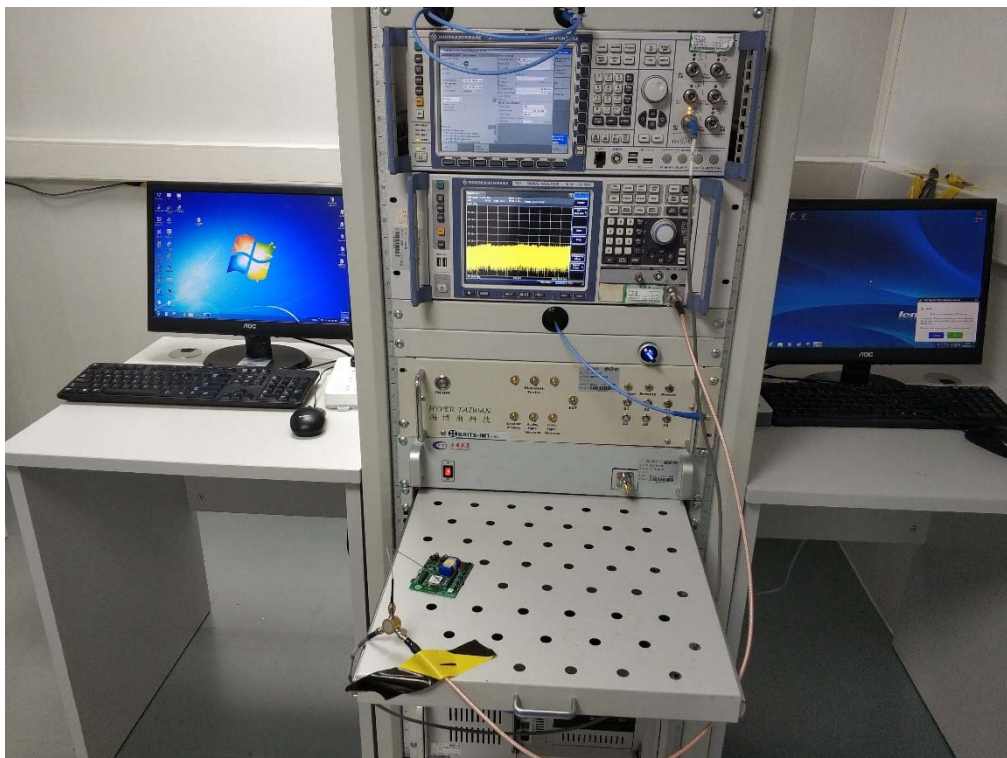
Conducted Test-BT
