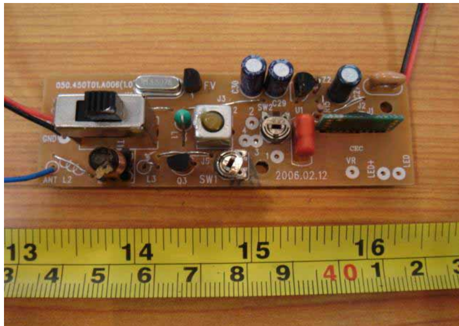
PCB - Front View
