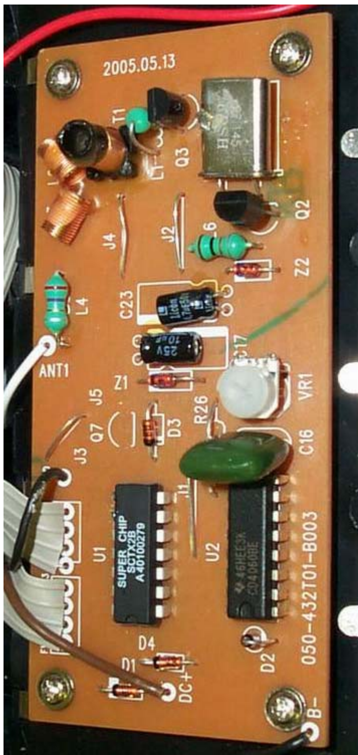
Component Side
