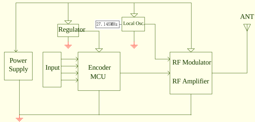
TX Block Diagram
