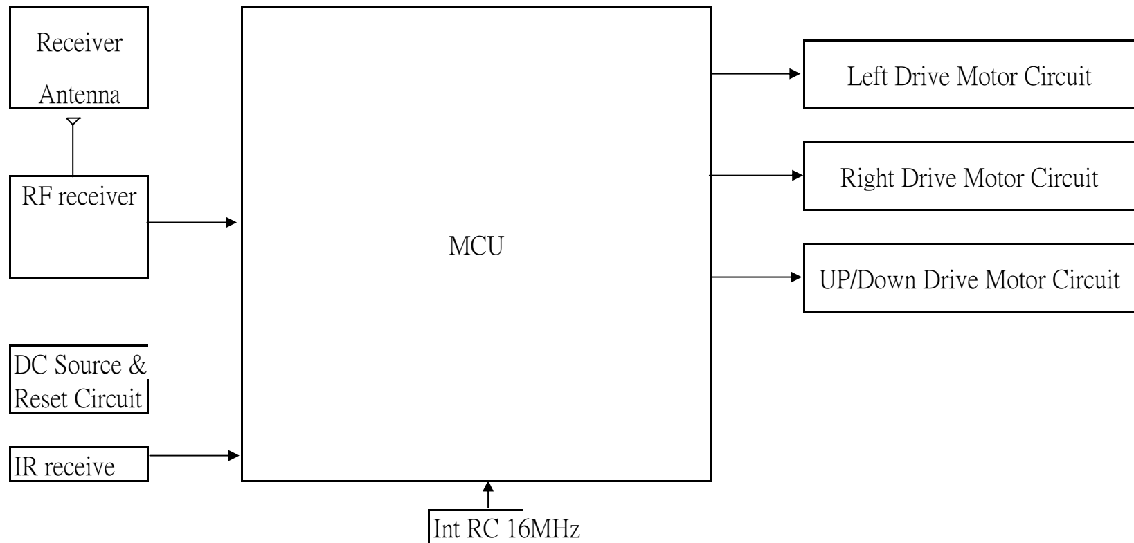
44008 I-FLY Rx Block Diagram
