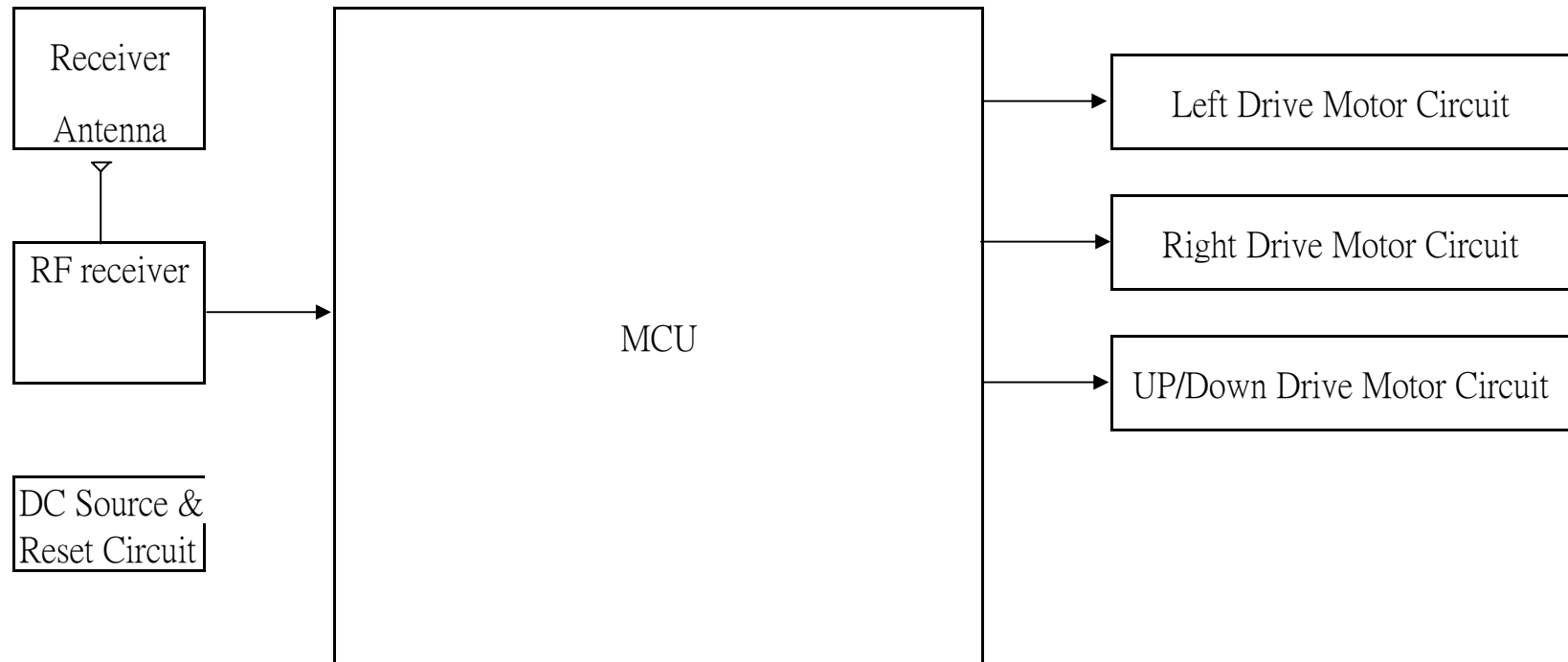
44008 I-FLY Rx Block Diagram
