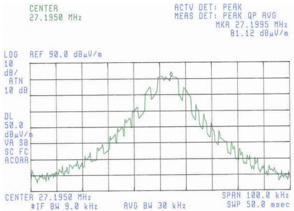
Figure 5.1 Bandwidth Plot
