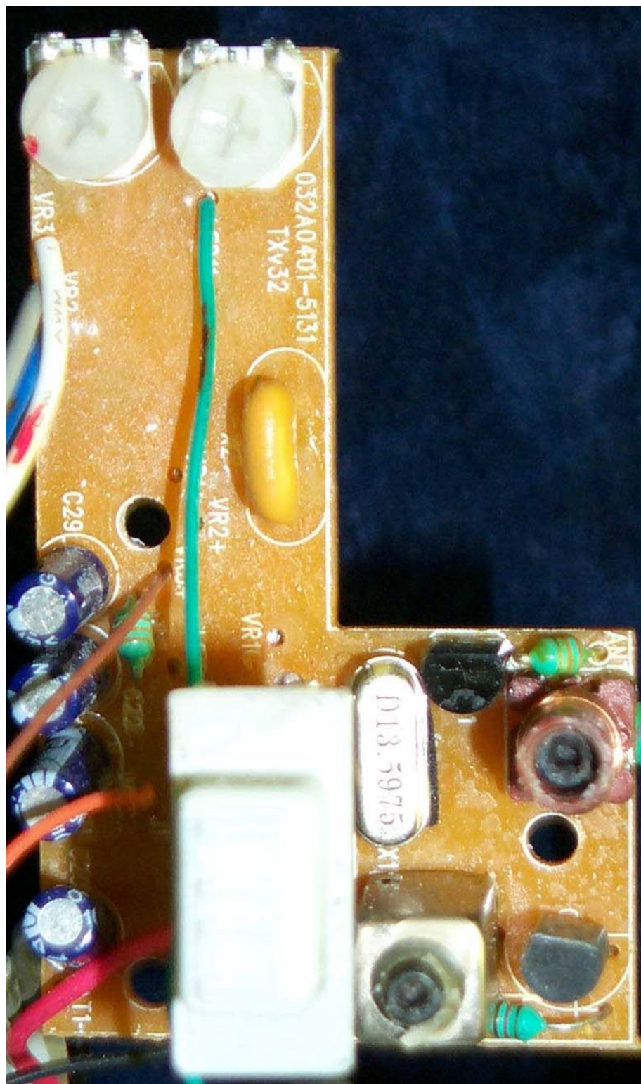
Component Side
