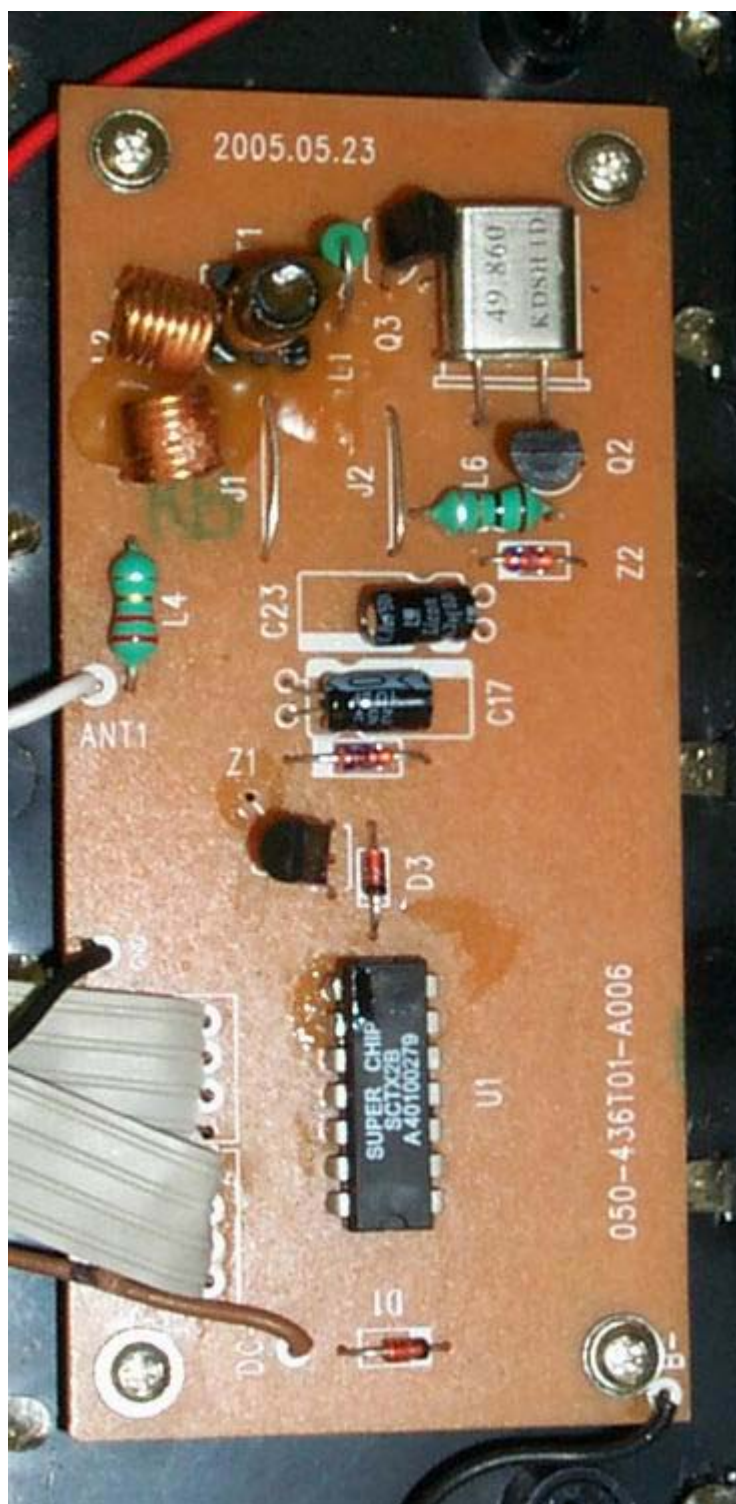
Component Side
