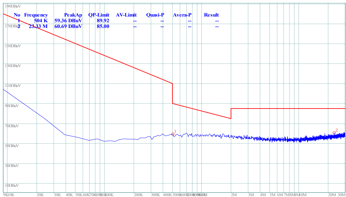
(Plot C.0: 9kHz to 30MHz @ 8-DPSK, channel 78)
