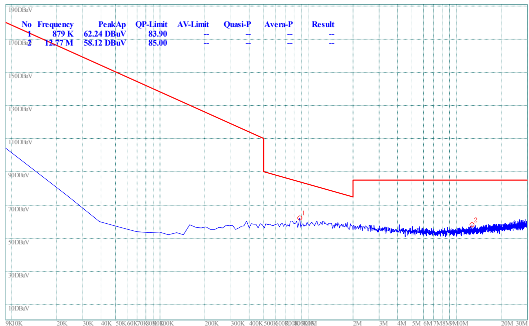
(Plot C.0: 9kHz to 30MHz @ GFSK, channel 78)
