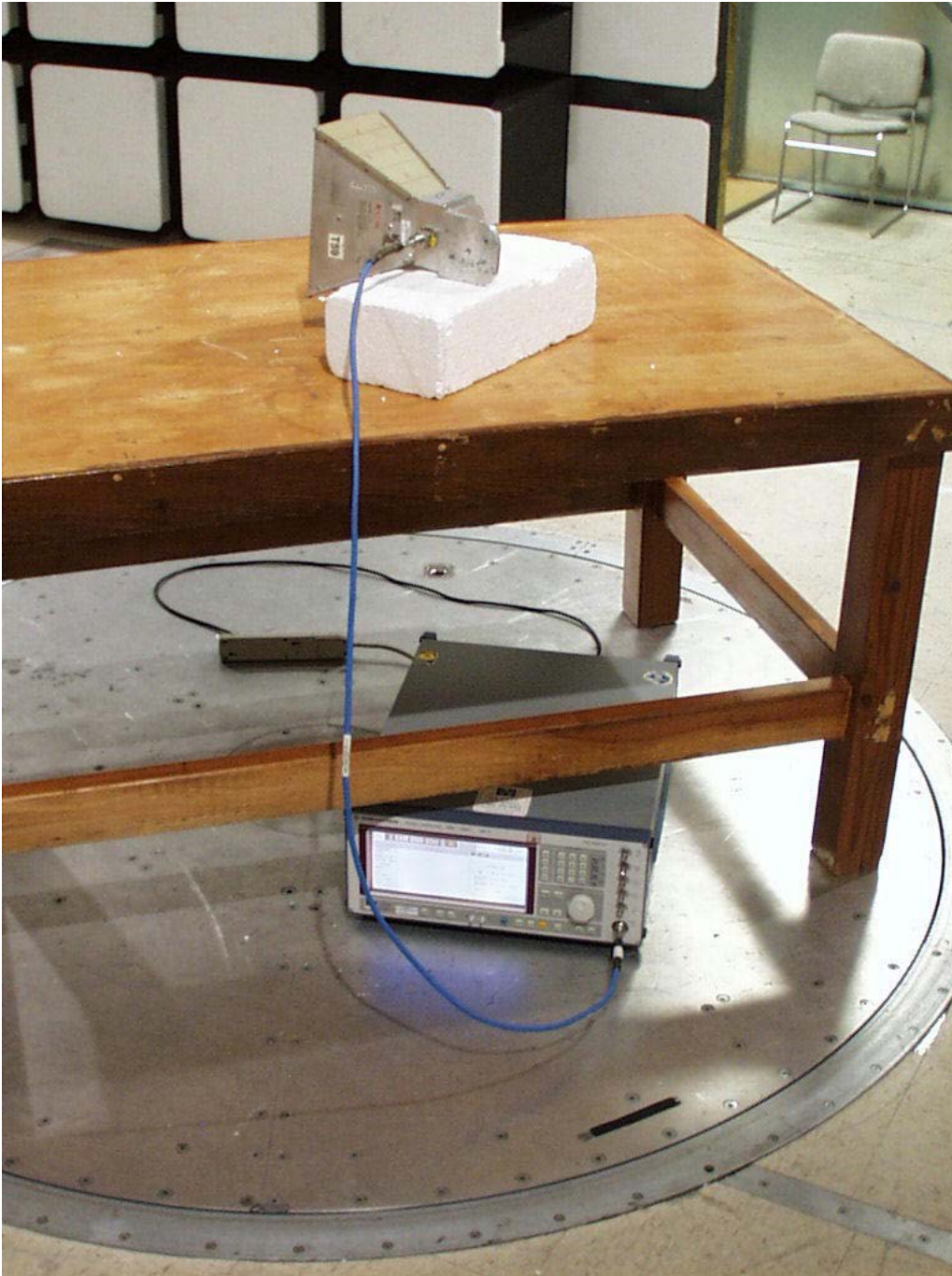
Signal generator and substitution antenna
