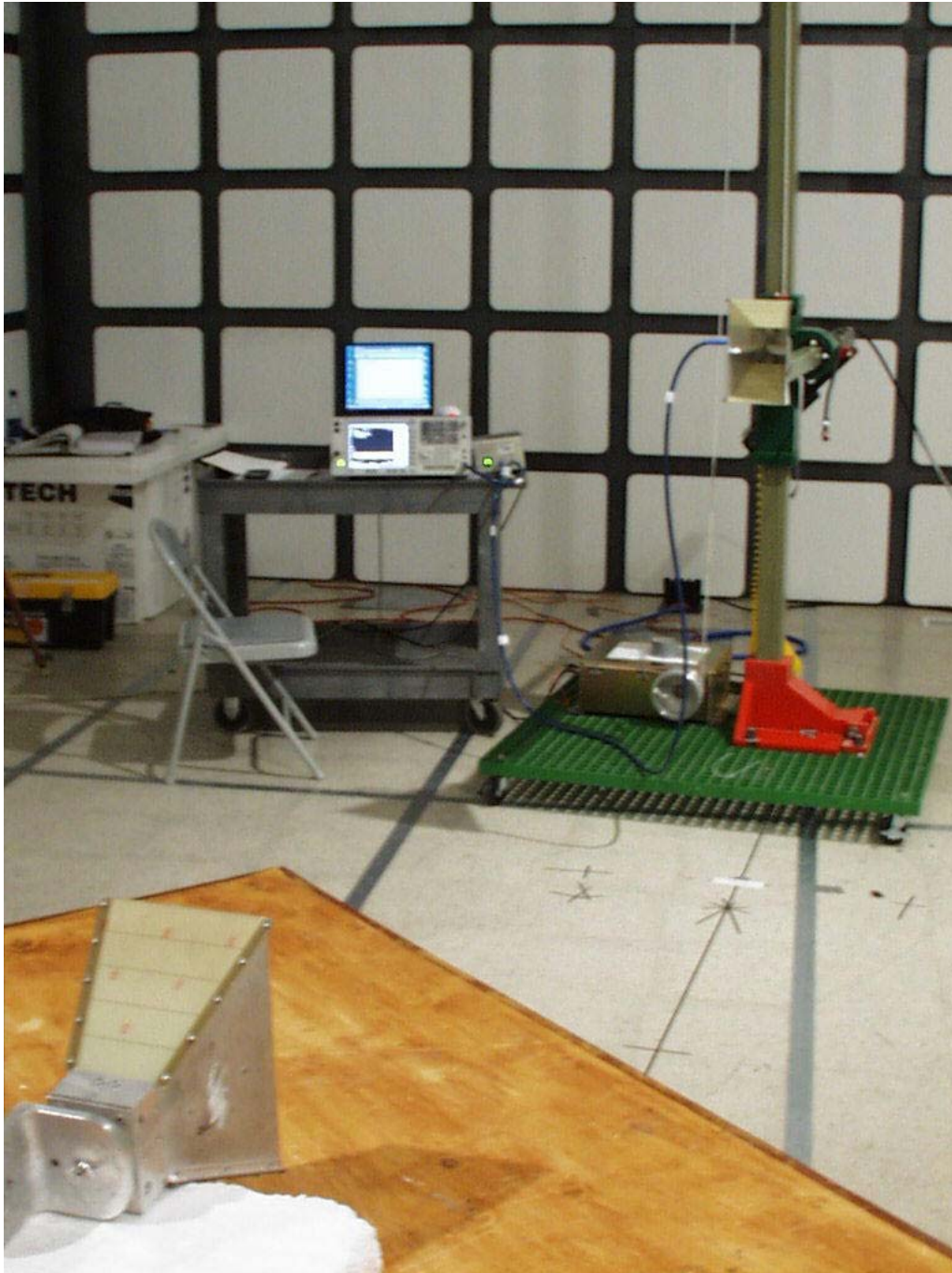
Substitution radiated test set-up
