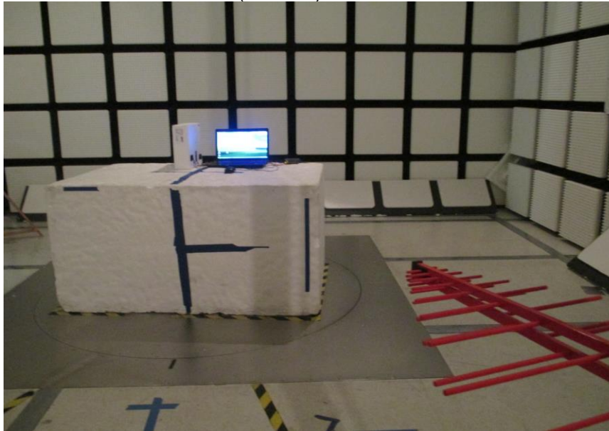
RADIATED EMISSIONS (FRONT)
