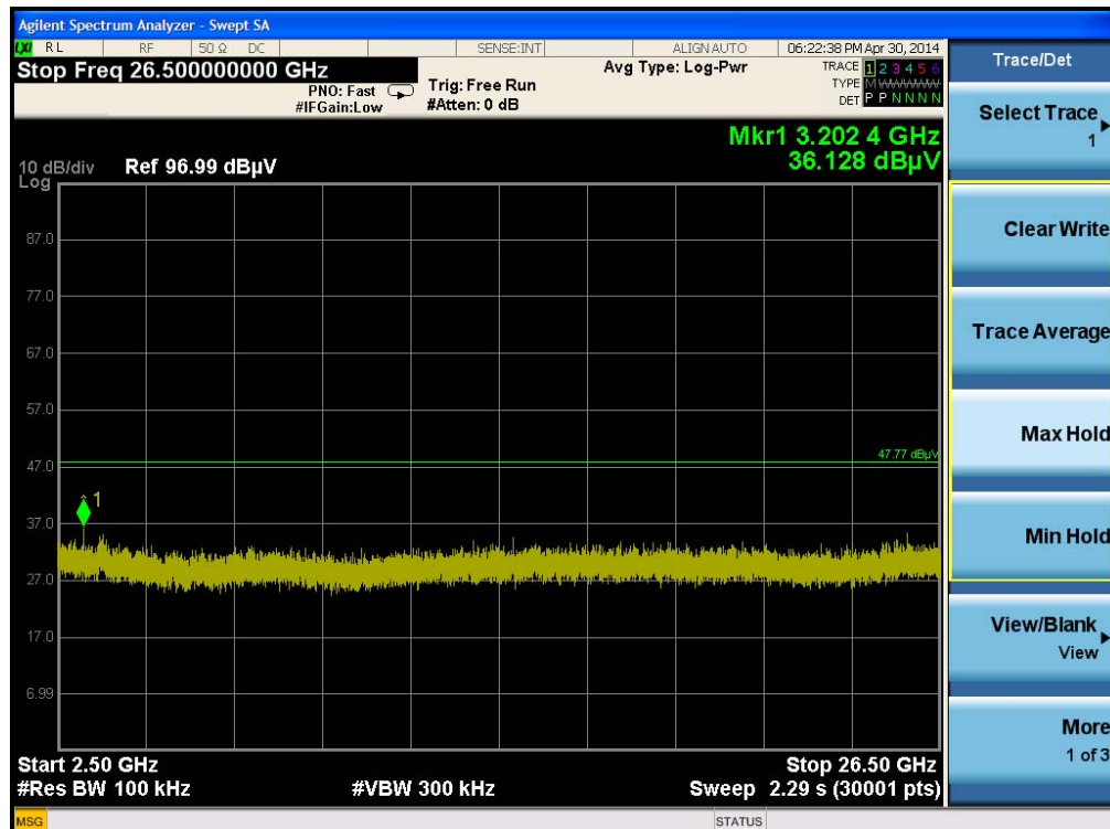
Plot on Configuration For EDR (8DPSK) / Channel 78 / Reference Level (Vertical)
