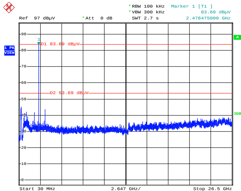
Plot on Configuration For EDR (8DPSK) / Channel 78 / Reference Level (Vertical)
