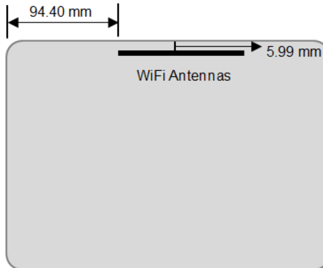
Antenna Location – Bottom View
