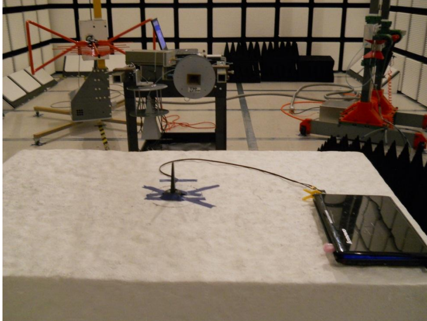
RADIATED BACK PHOTO (From 18 GHz – 40GHz)
