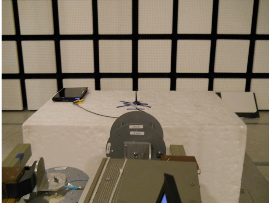
RADIATED FRONT PHOTO (From 18 GHz – 40GHz)
