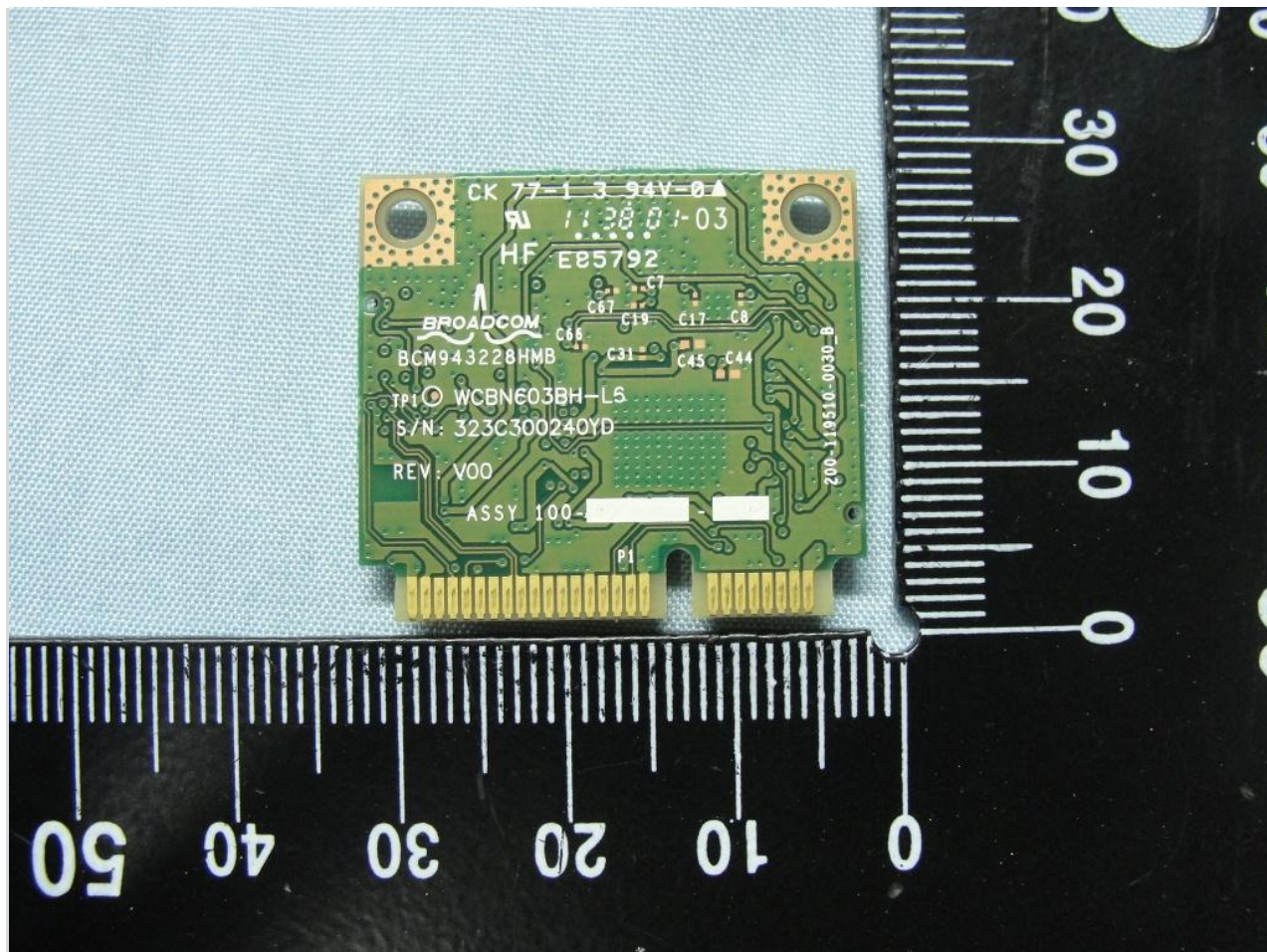
EUT: WLAN module (Broadcom / BCM943228HMB)
