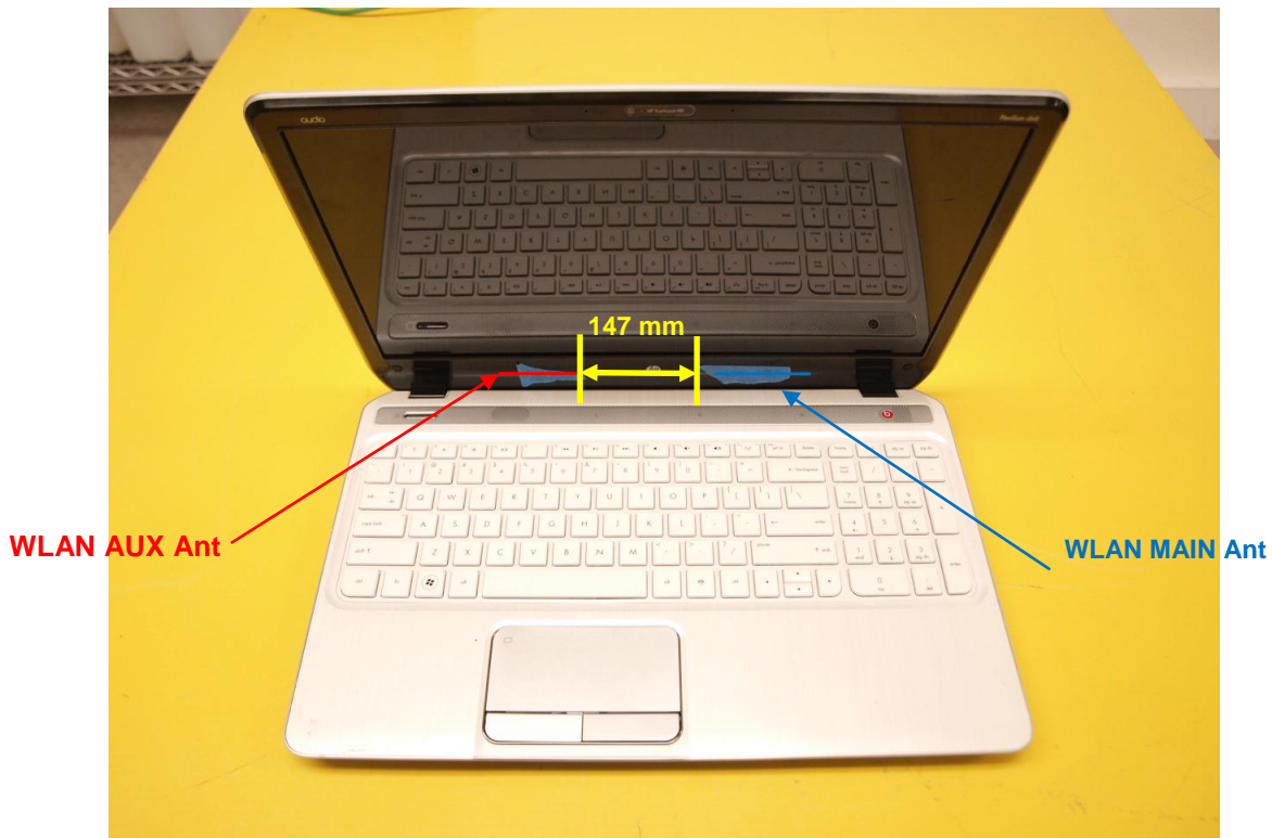
Lap-held configuration (Separation distance between antenna and user)
