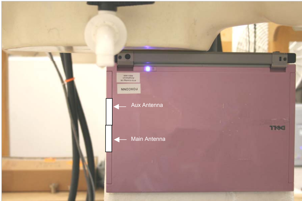
Setup Photo with SAM Phantom (2.4 GHz band)
