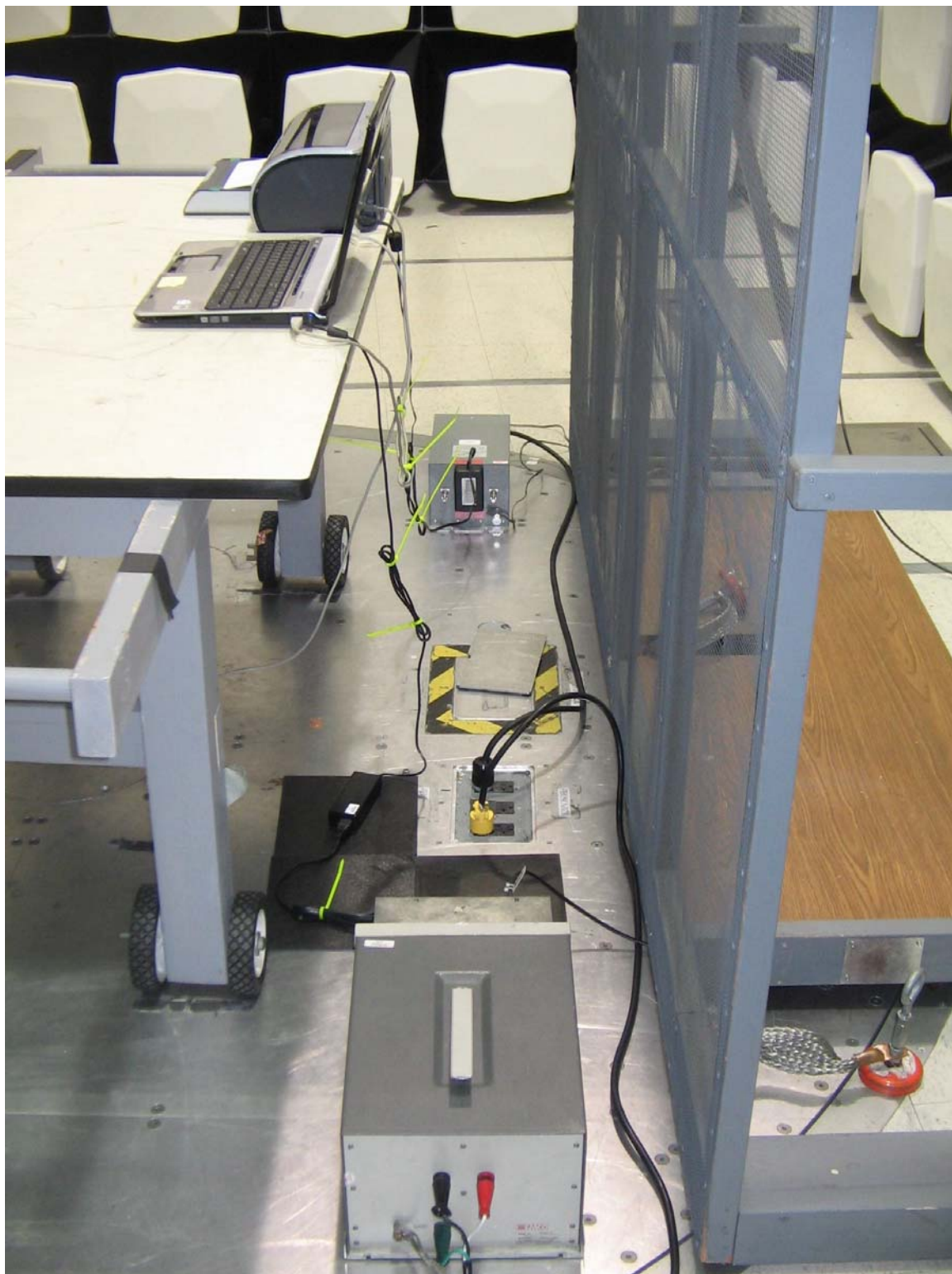
Conducted Emissions Test Configuration Photographs
