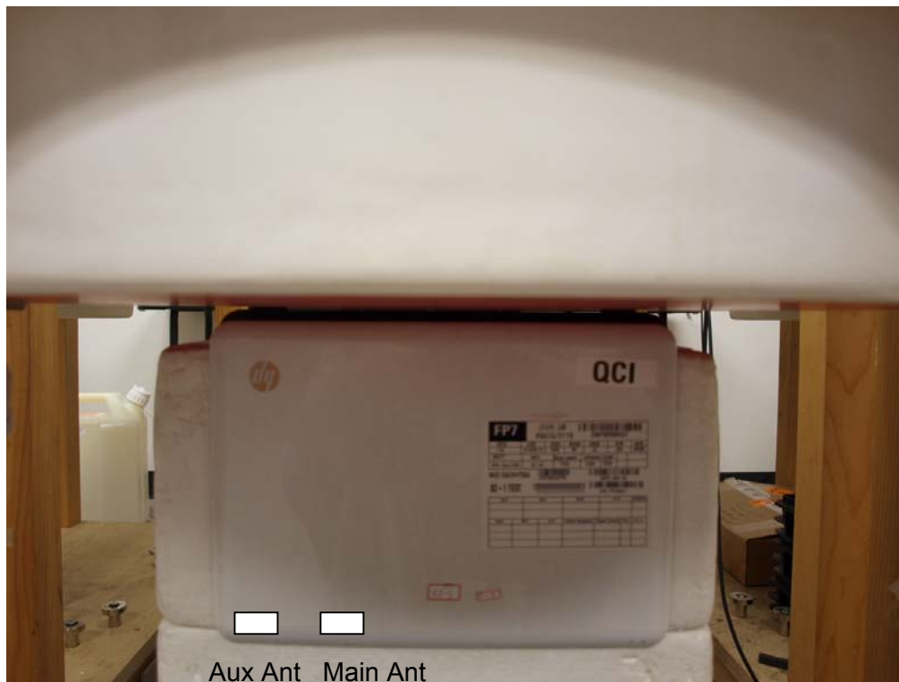
SAR TEST SETUP PHOTO
