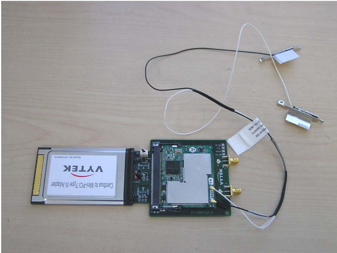
WLAN in Test fixture with Antenna
