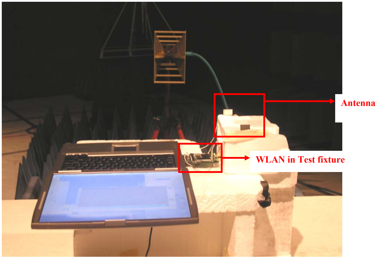
Test setup – Radiated measurements
