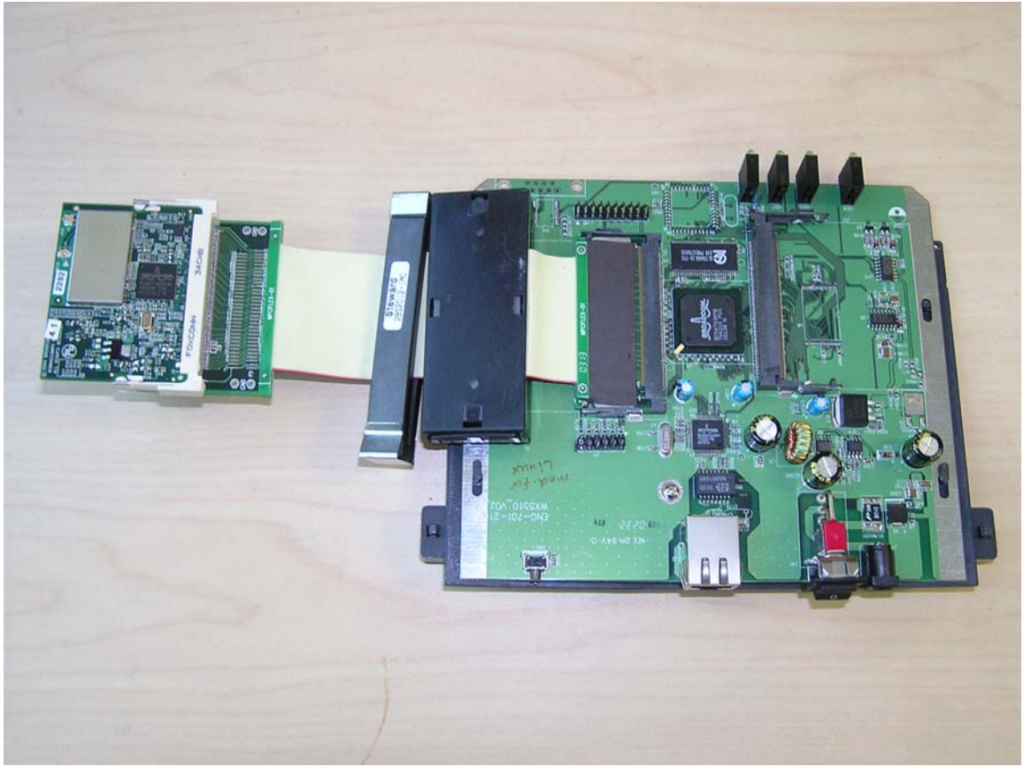
Test fixture with WLAN Top
