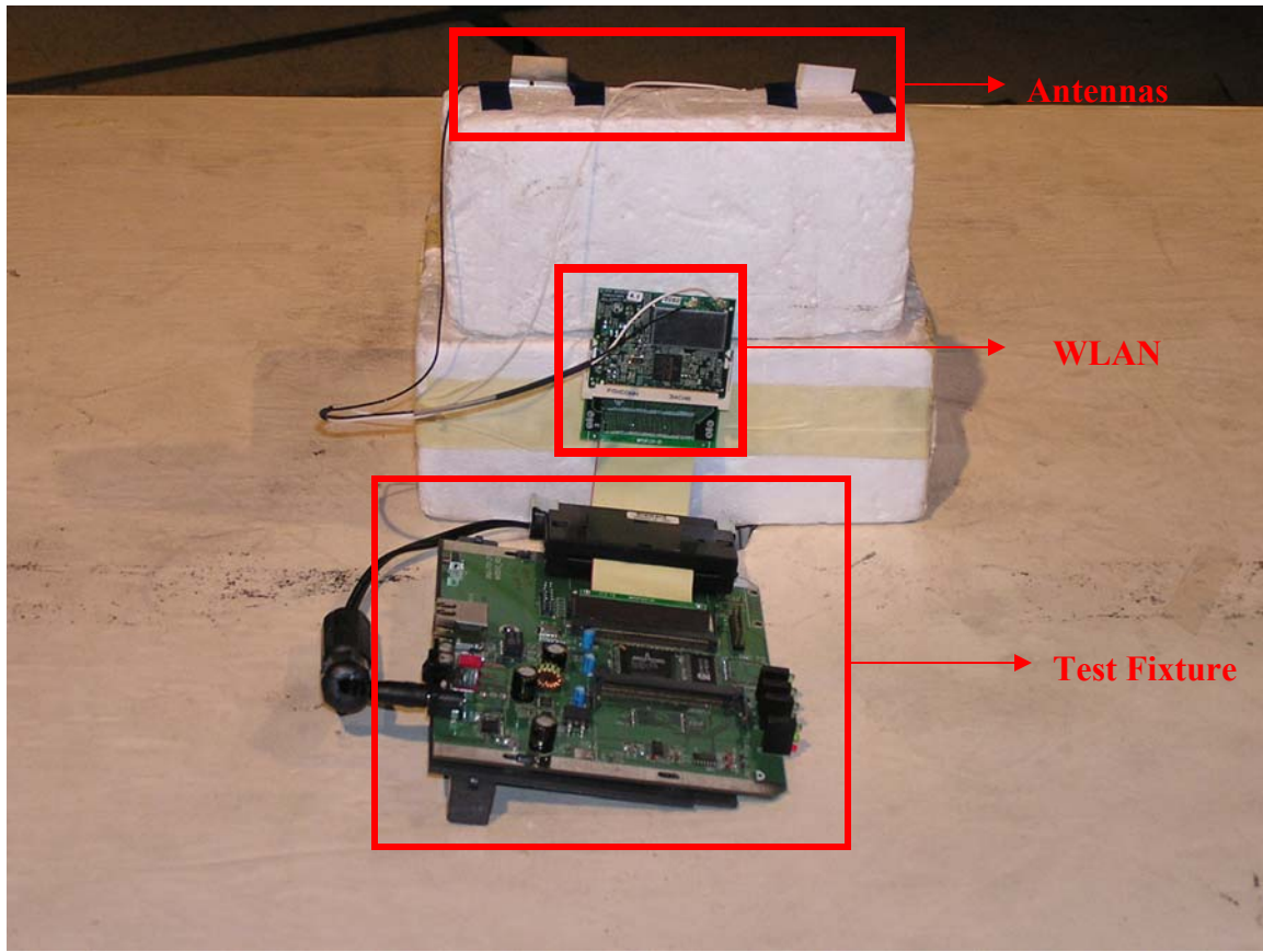
Test setup – Radiated measurements (showing test fixture with WLAN)
