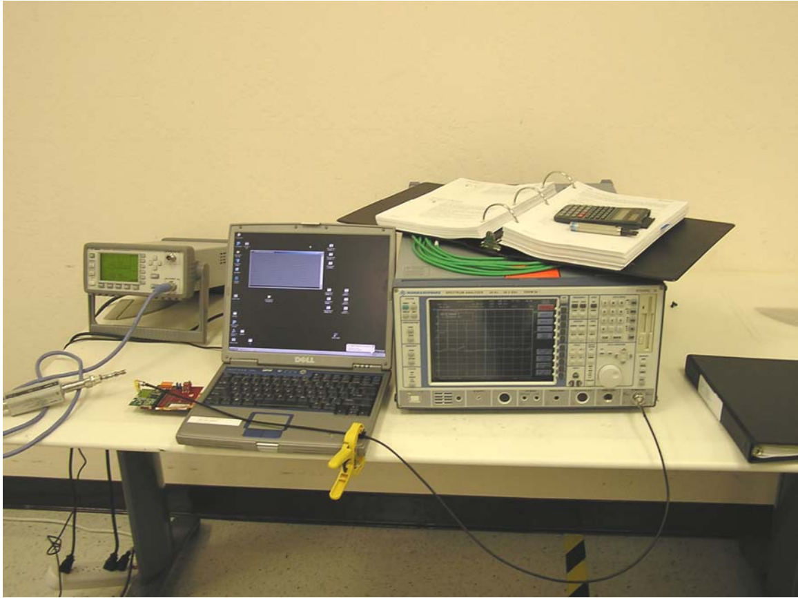
Test setup – Conducted measurements (Different setup was used only for conducted measurements)
