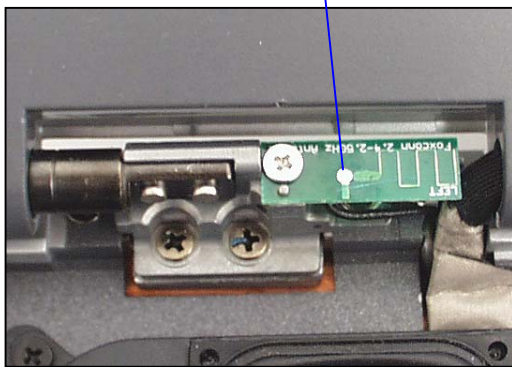
LEFT ANTENNA
