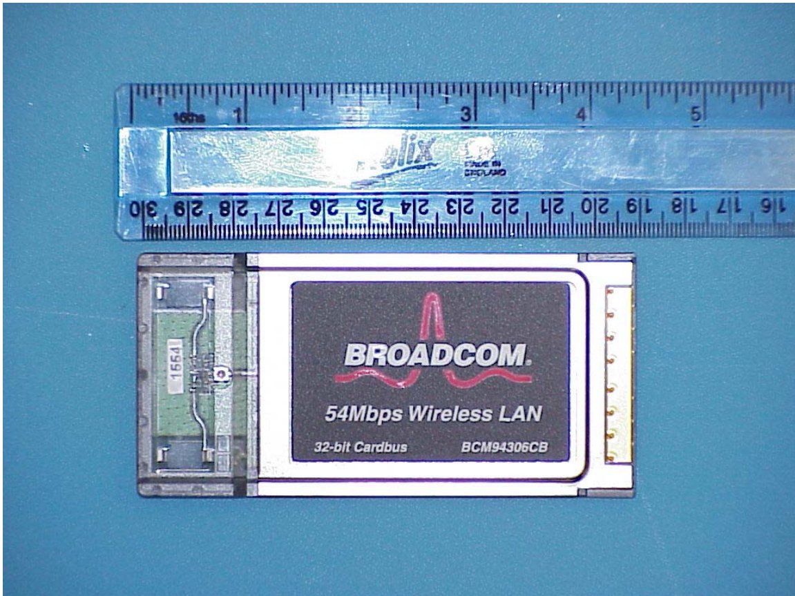
Photo 1. EUT front
