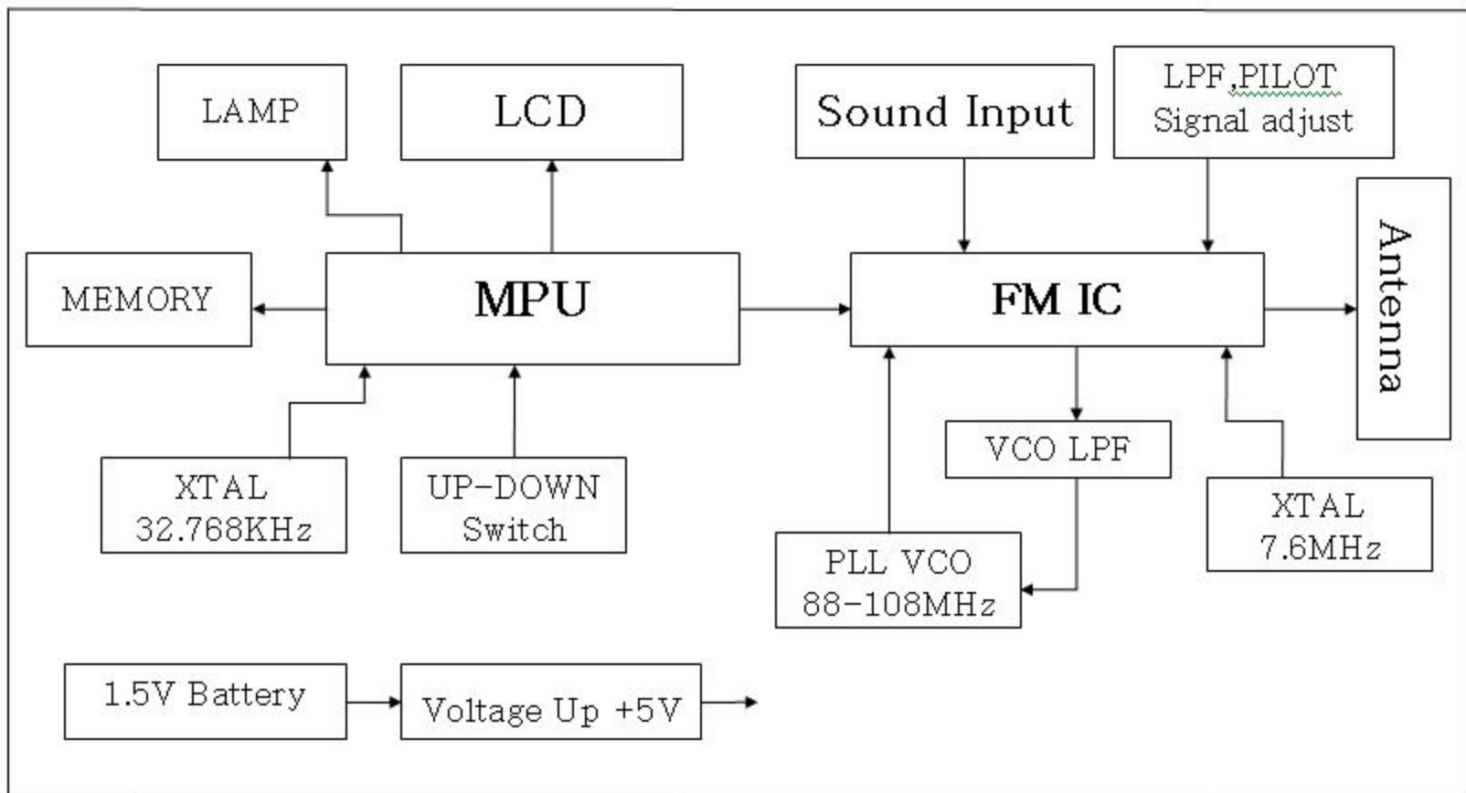
FM Linker Block Diagram
